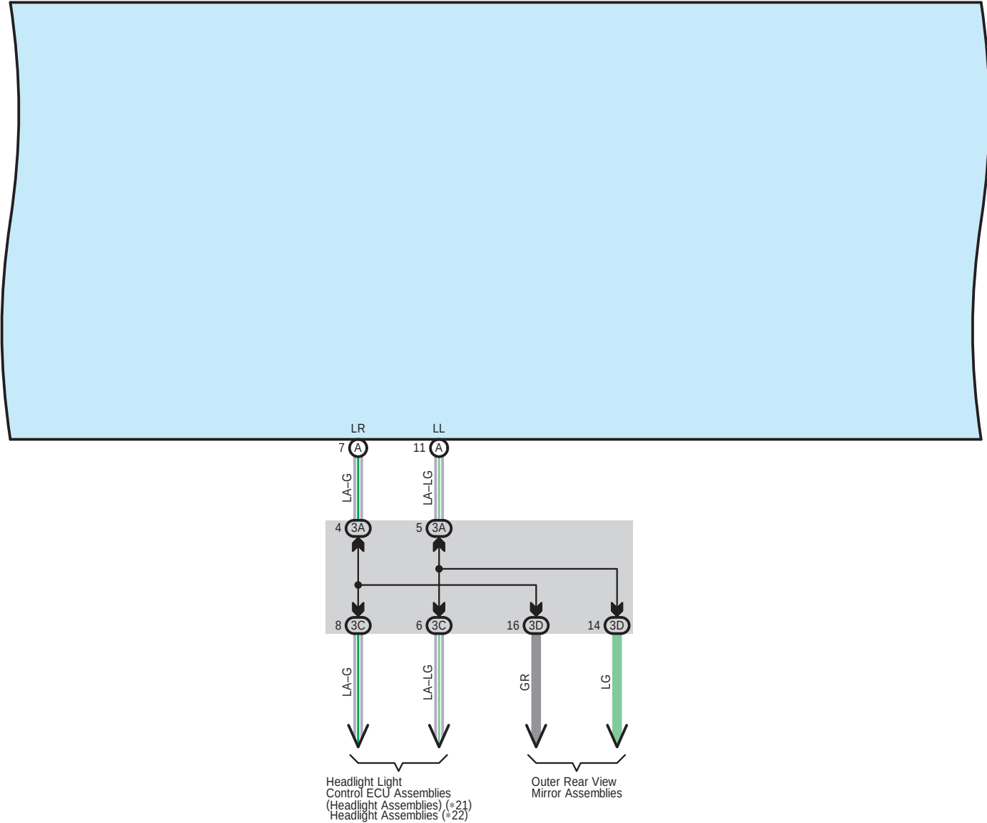
K20(A), K21(B) Combination Meter Assembly
