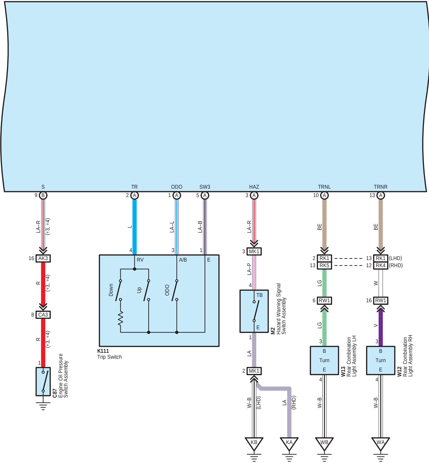
K20(A), K21(B) Combination Meter Assembly
