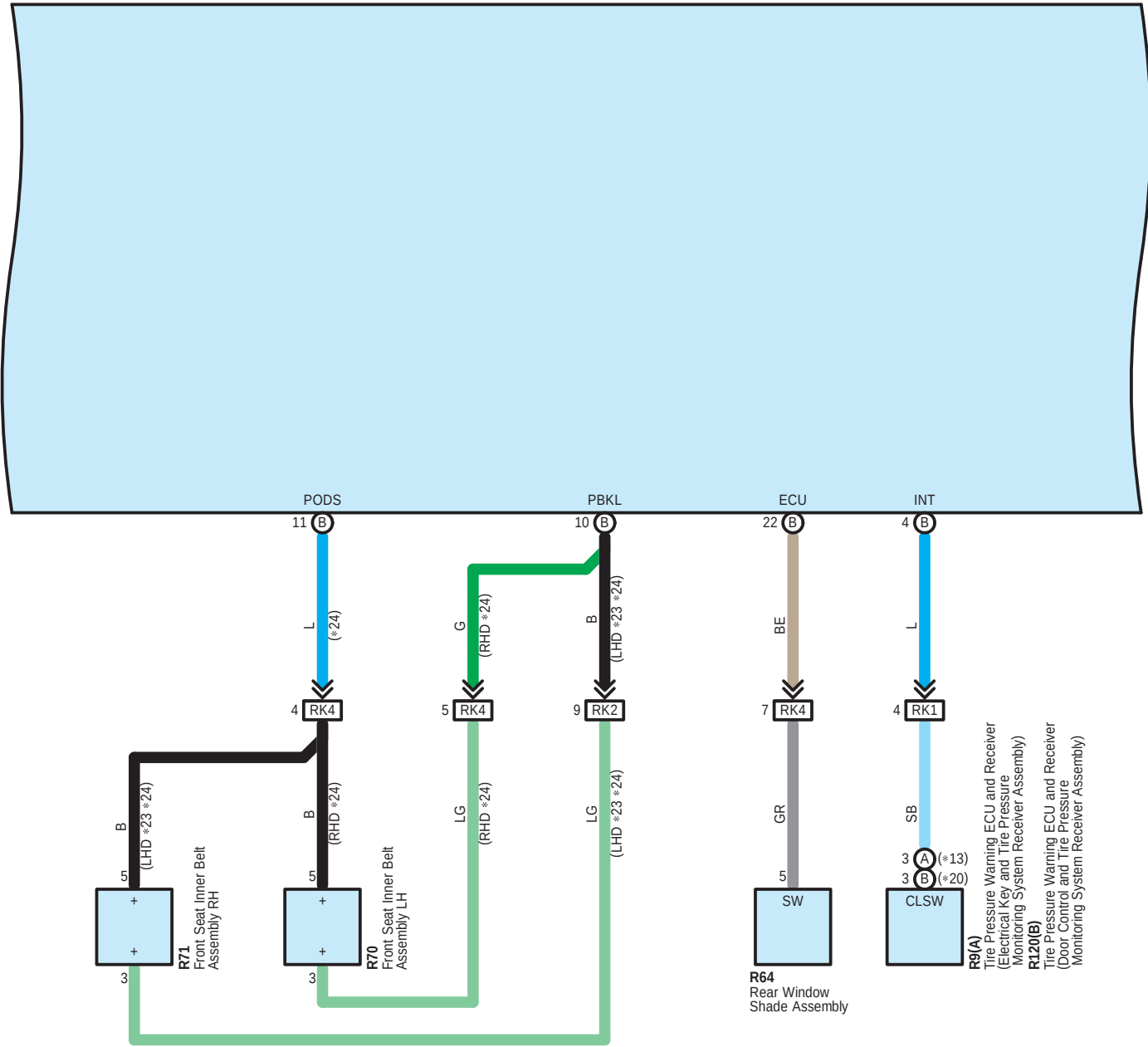
K20(A), K21(B) Combination Meter Assembly
