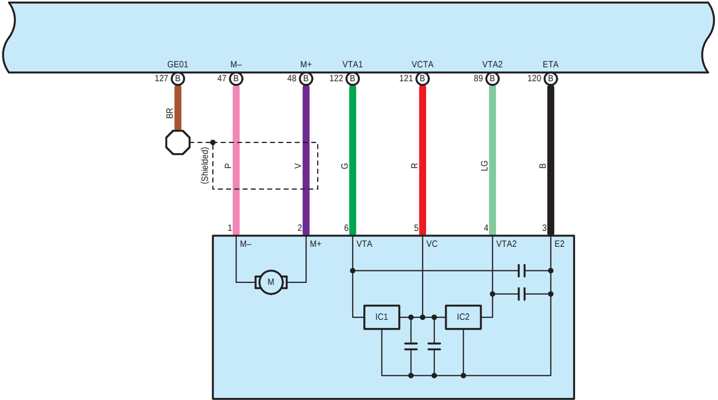
C82 Throttle with Motor Body Assembly
