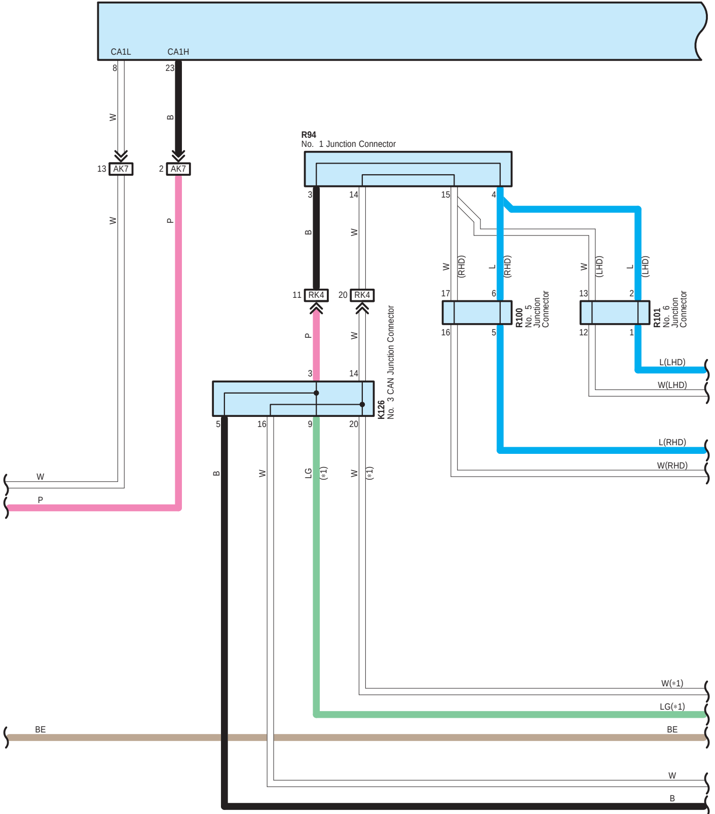
K76 Network Gateway ECU (Central Gateway ECU)
