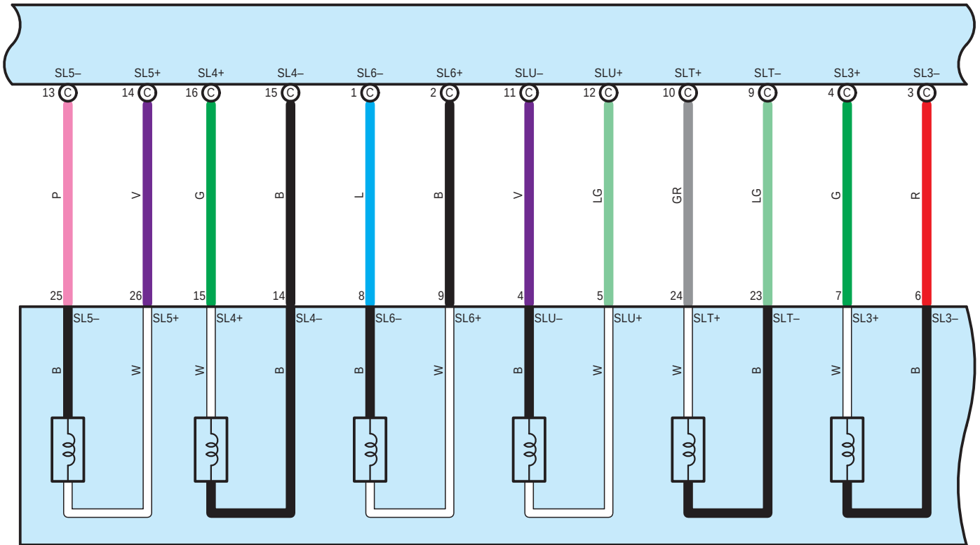
C93 ECT Solenoid (Transmission Wire)
