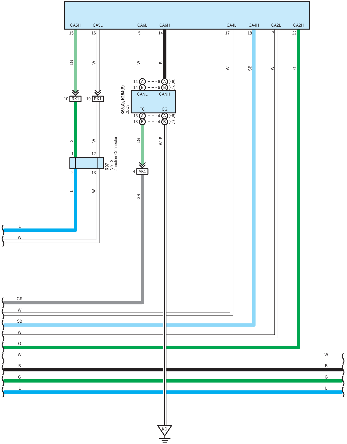
K76 Network Gateway ECU (Central Gateway ECU)
