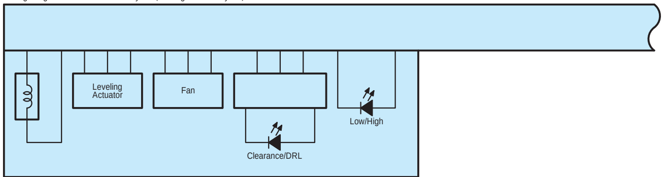
A10 Headlight Light Control ECU Assembly LH (Headlight Assembly LH)
