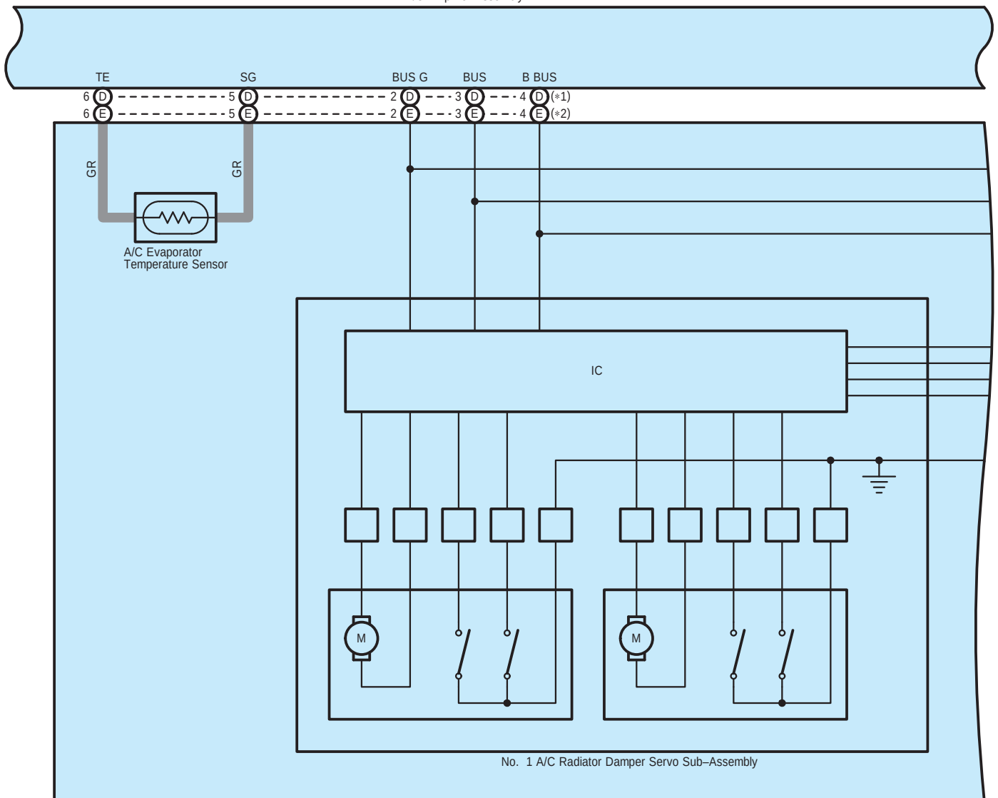
z8(D), z11(E) A/C Unit (A/C Harness Assembly)
