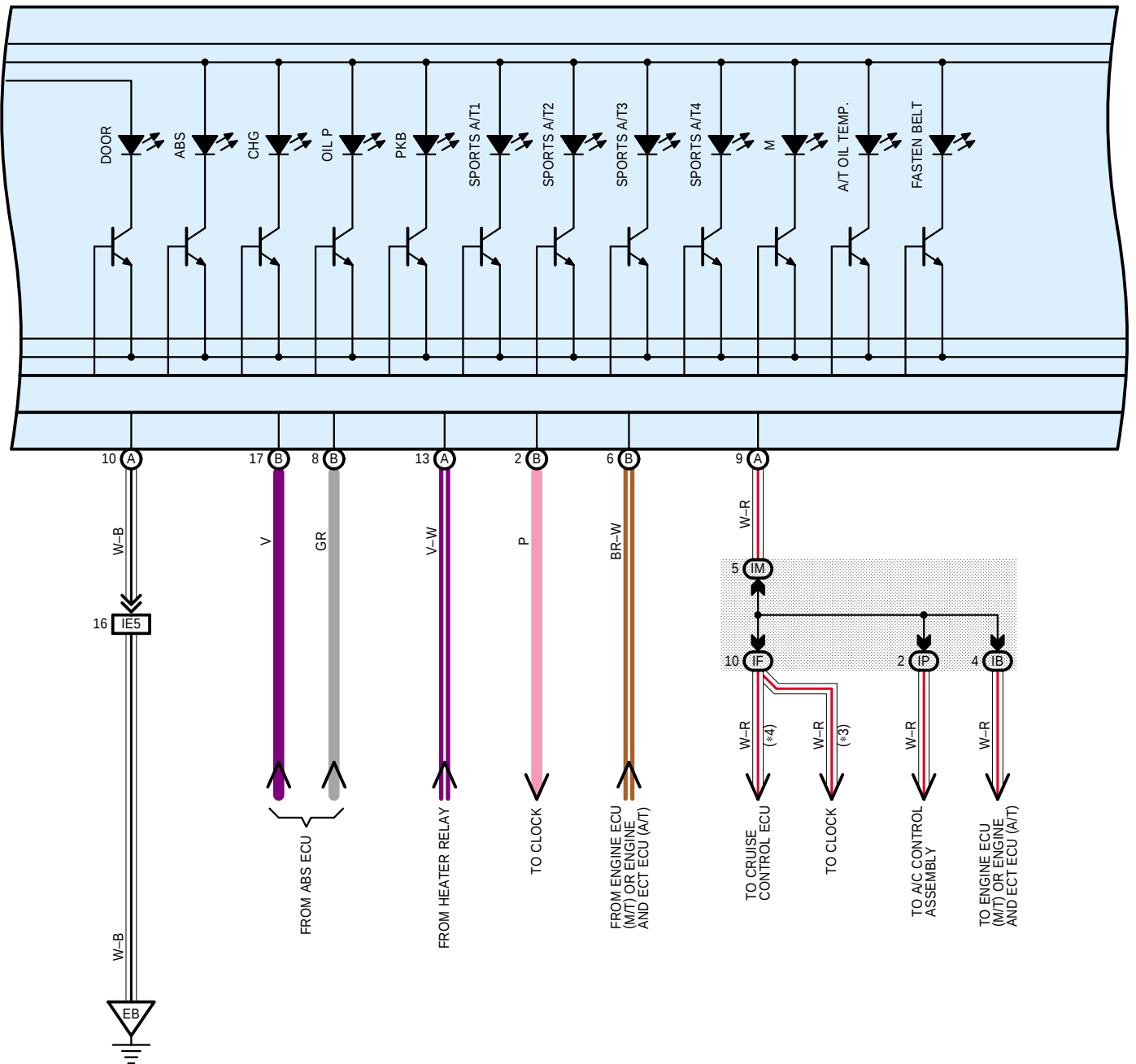
C11 (A), C12 (B) COMBINATION METER
