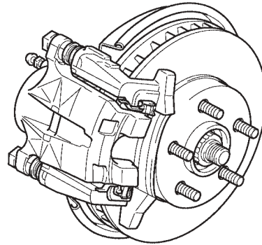
15 inch Disc (2ZZ-GE Engine Model)
