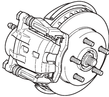
14 inch Disc (1ZZ-FE Engine Model)
