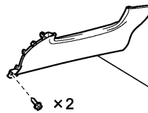
LOWER INSTRUMENT PANEL FINISH PANEL SUB-ASSEMBLY
