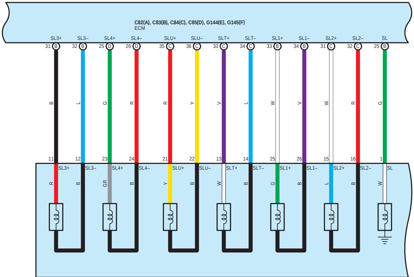
C31 ECT Solenoid (Transmission Wire)
