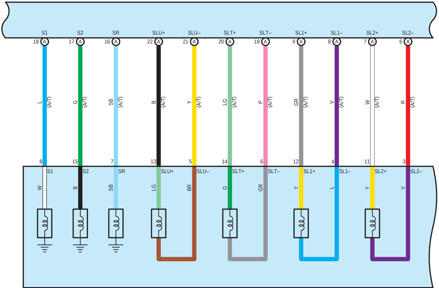
C132 ECT Solenoid (Transmission Wire)
