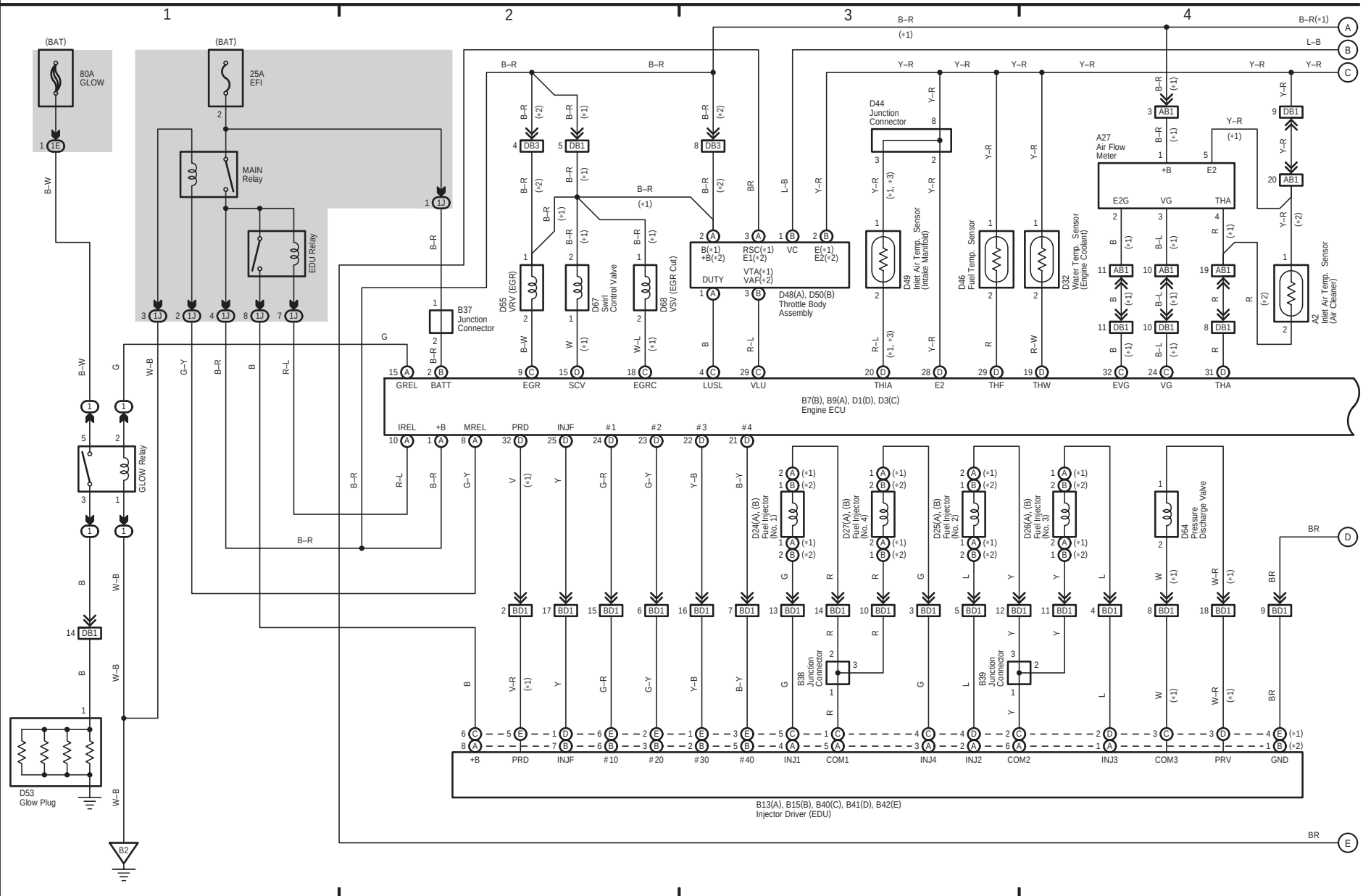
Engine Control (1KD-FTV Before Aug. 2010 Production, 2KD-FTV)
