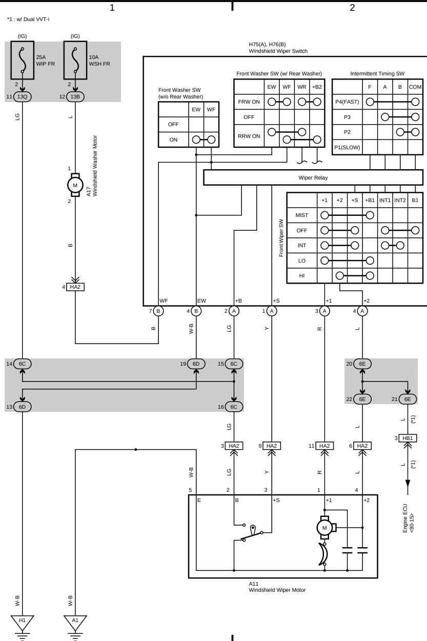
Front Wiper and Washer (LHD) (From Dec. 2013 Production)
