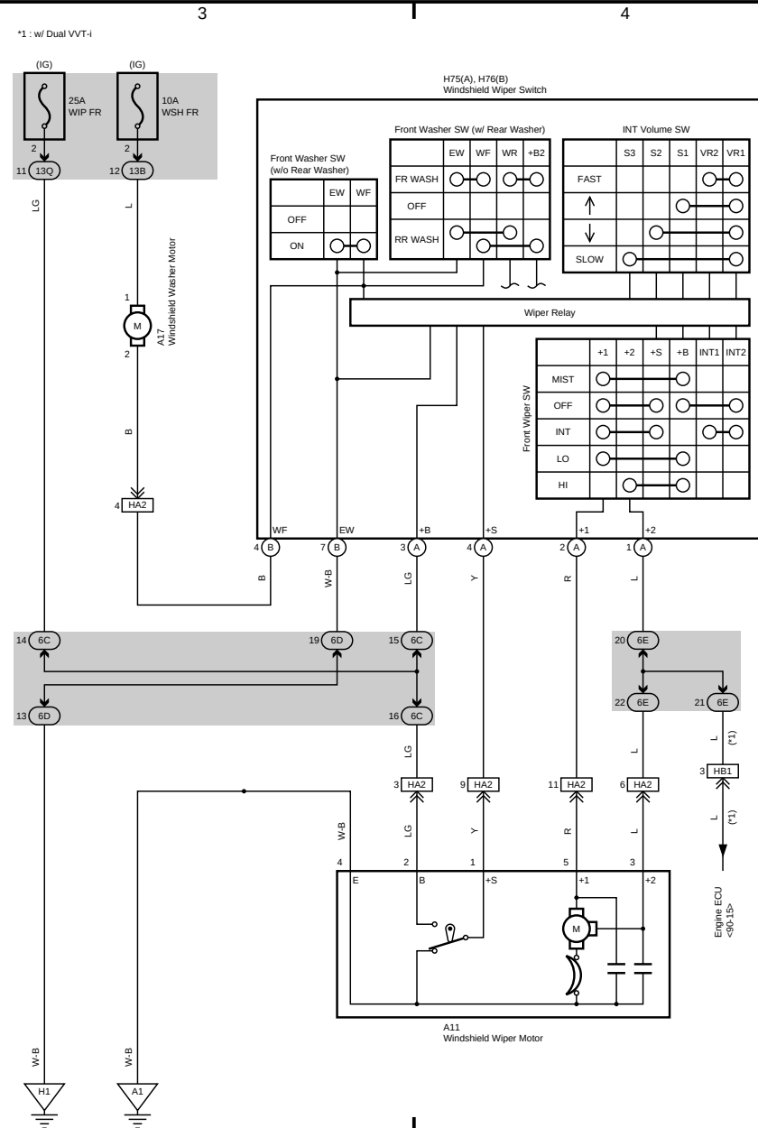
Front Wiper and Washer (RHD) (From Dec. 2013 Production)
