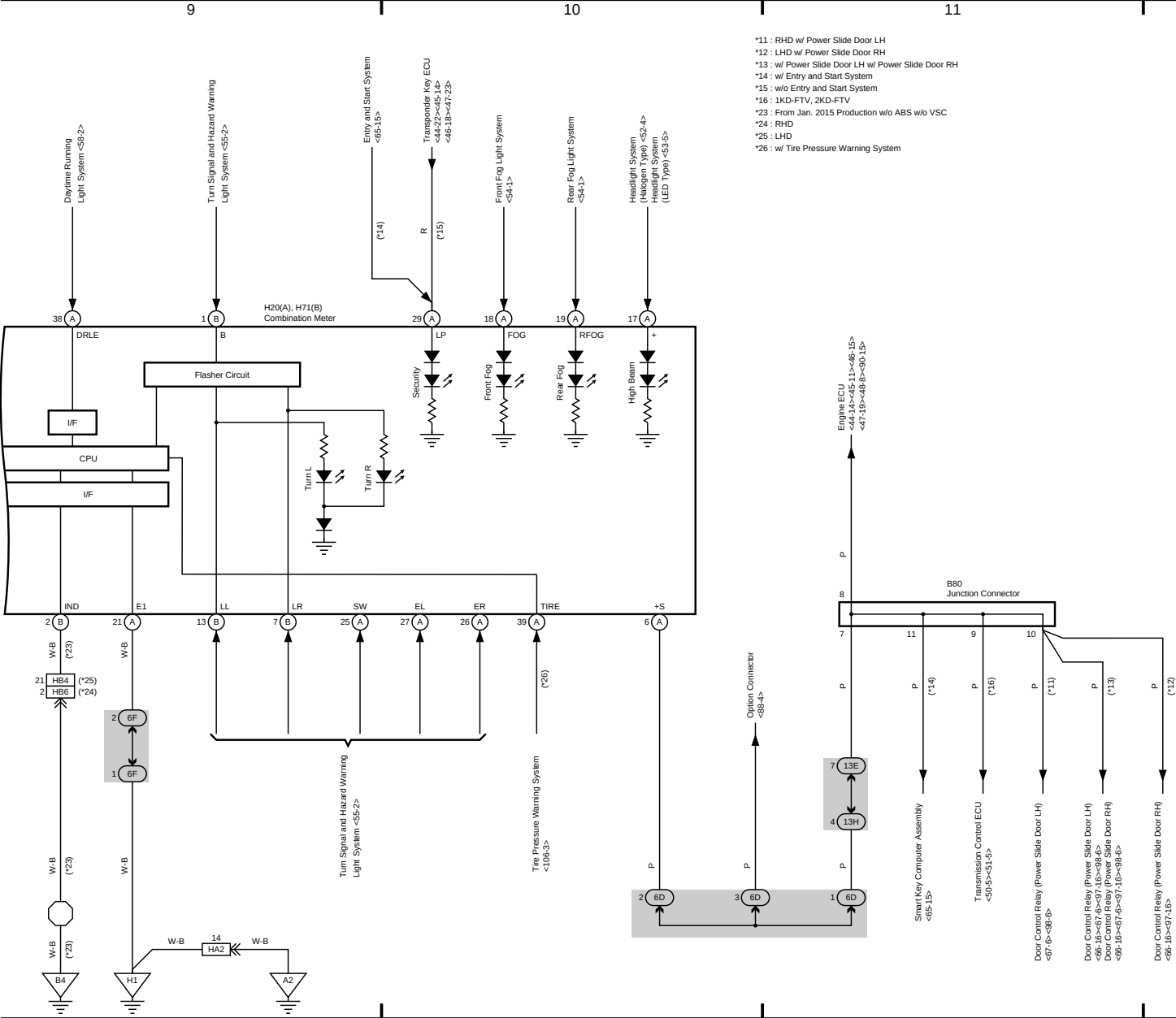
Combination Meter (From Dec. 2013 Production) (Except 1GD-FTV) and Clock (From Dec. 2013 Production) (Except 1GD-FTV)
