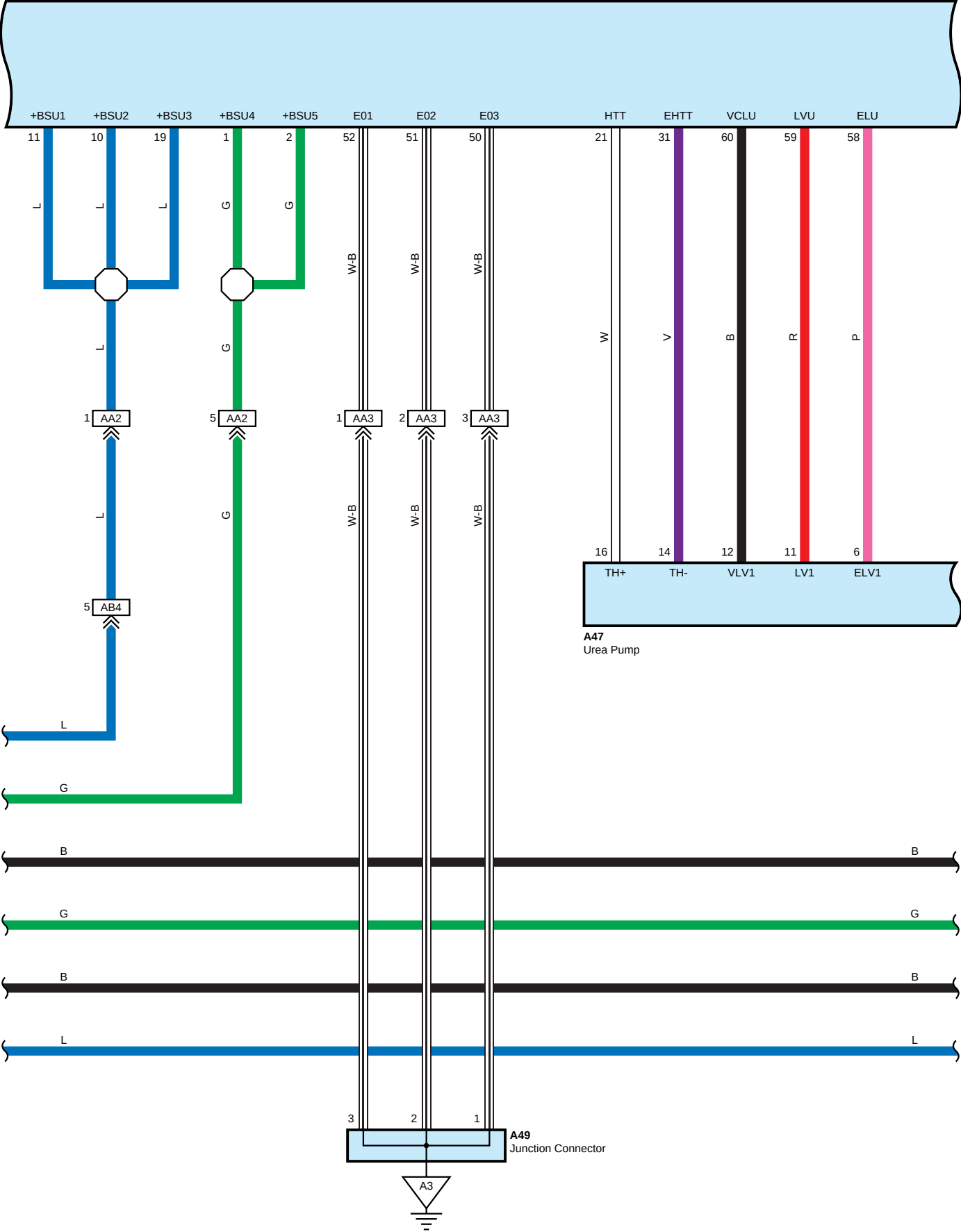
A45 Urea Pump Control ECU
