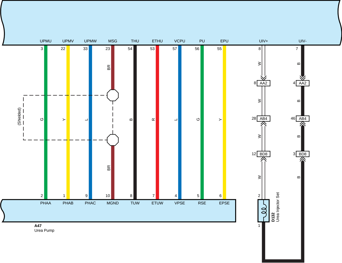
A45 Urea Pump Control ECU
