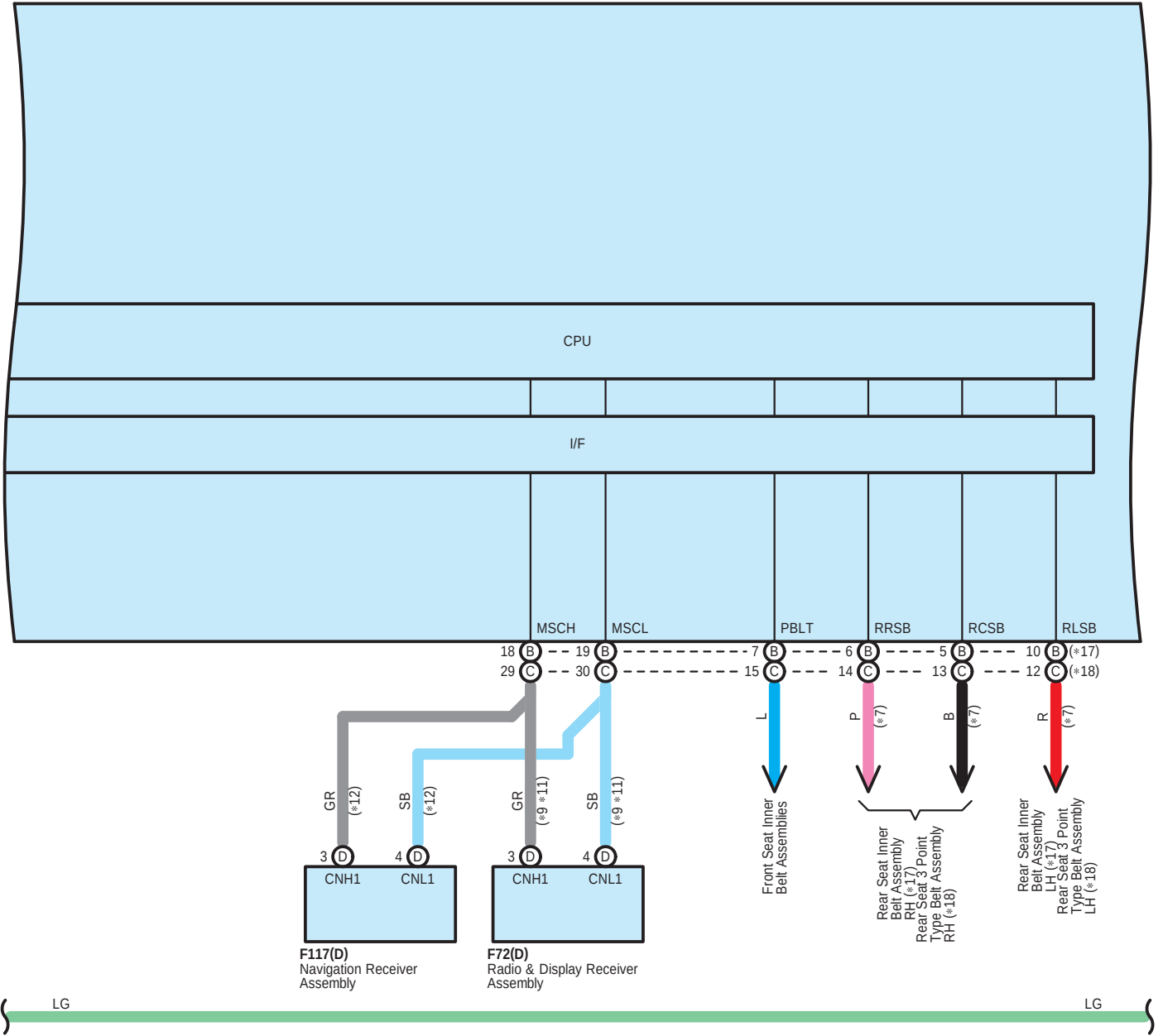
F21(A), F22(B), F126(C) Combination Meter Assembly
