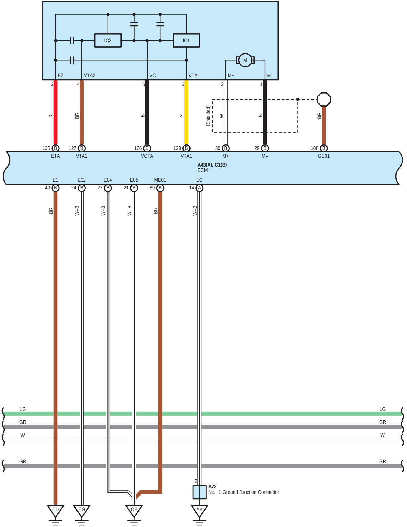
C41 Throttle Body with Motor Assembly
