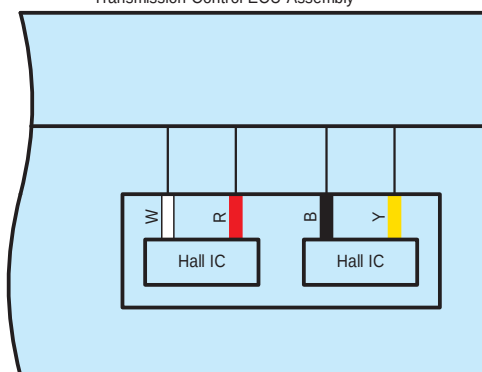
C3 Transmission Control ECU Assembly
