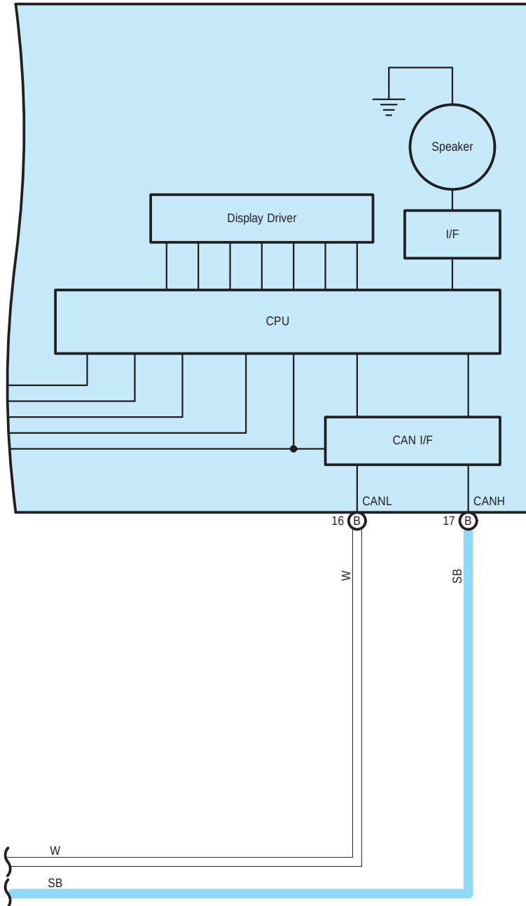
F22(B) Combination Meter Assembly
