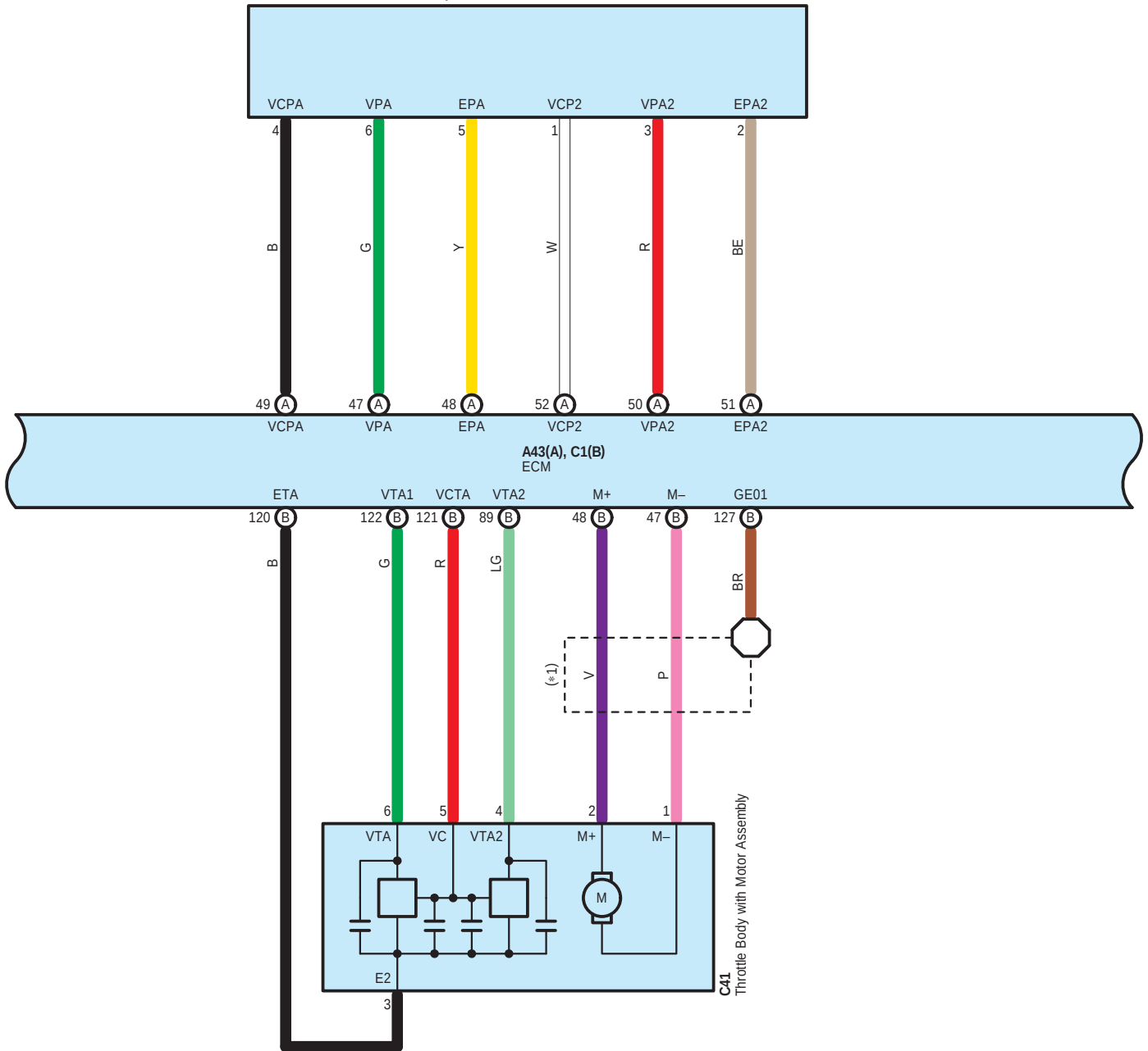
A53 Accelerator Pedal Sensor Assembly
