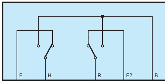
e11 Seat Variable Cushion Switch
