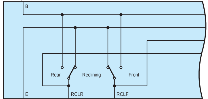
e5 Front Power Seat Switch LH
