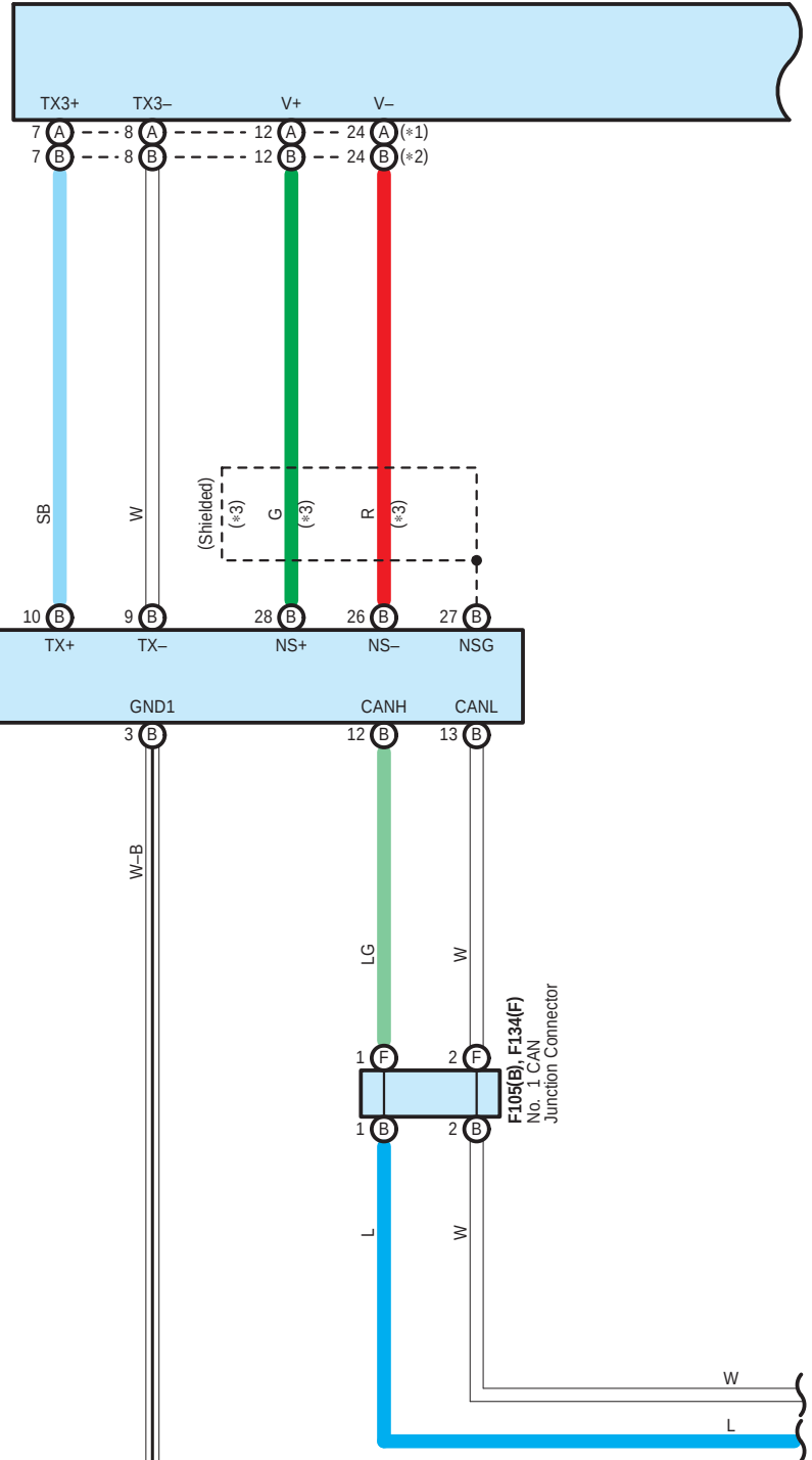
F71(C), F72(A) Radio & Display Receiver Assembly F116(D), F117(B) Navigation Receiver Assembly
