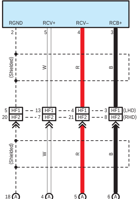
H18 Side Television Camera Assembly RH
