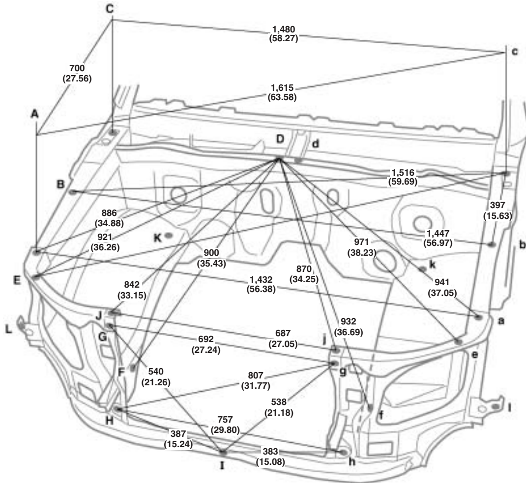
Vehicle Dimensions
