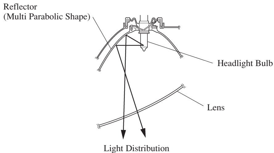
Multi-Reflector Type Headlight
