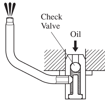
Oil Jet Cross Section
