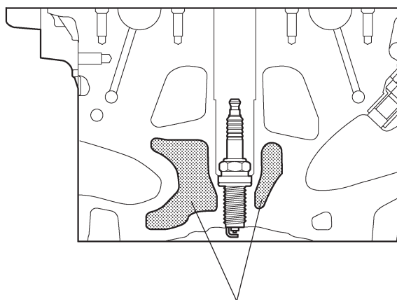
Water Jacket
