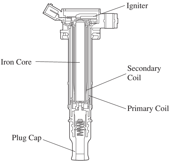
Ignition Coil Cross Section
