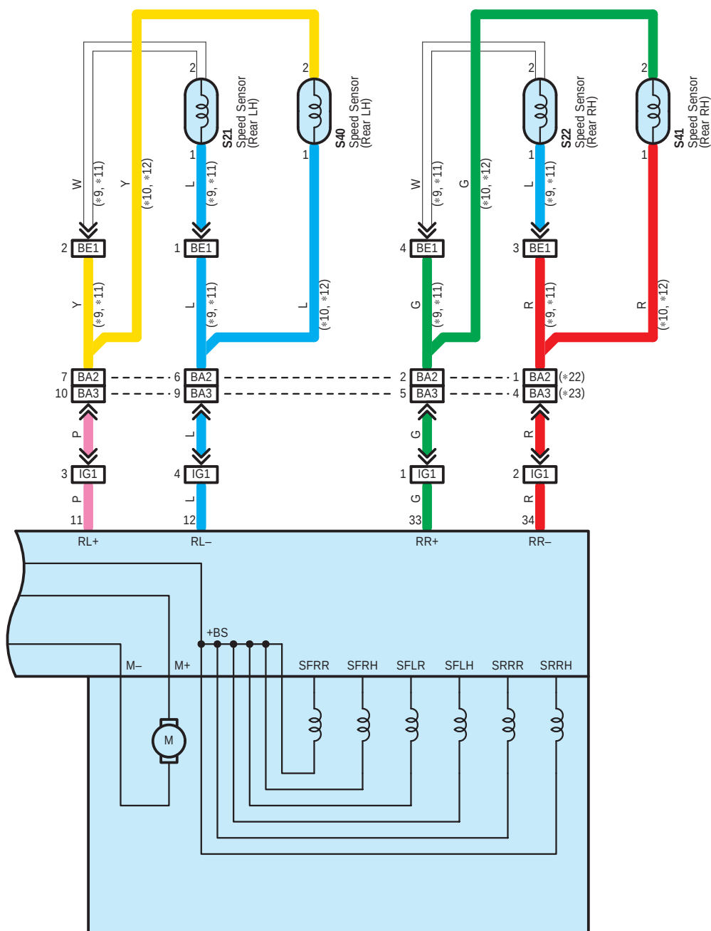
S 2 Skid Control ECU with Actuator
