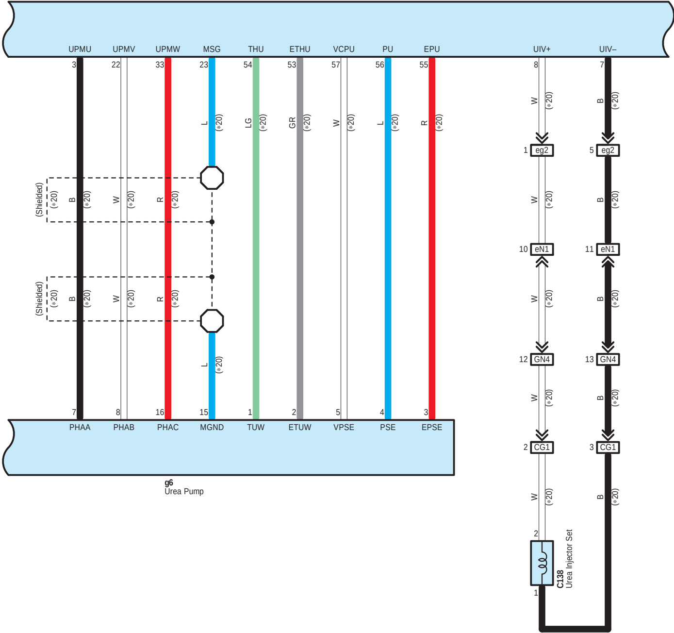
g1 Urea Pump Control ECU
