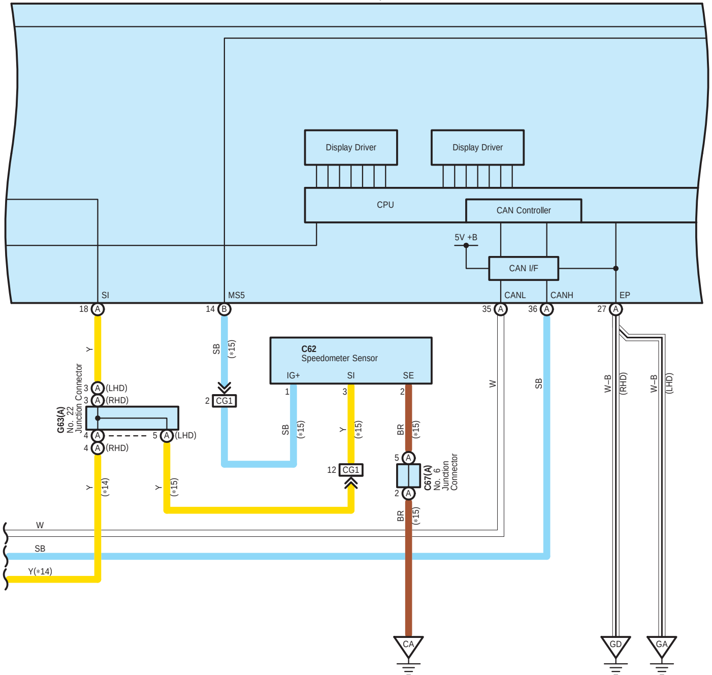
G9(A), G10(B) Combination Meter Assembly
