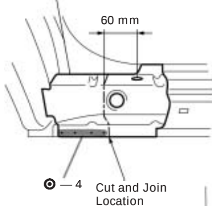
Rocker Panel Reinforcement
