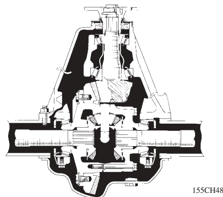
Rear Differential
