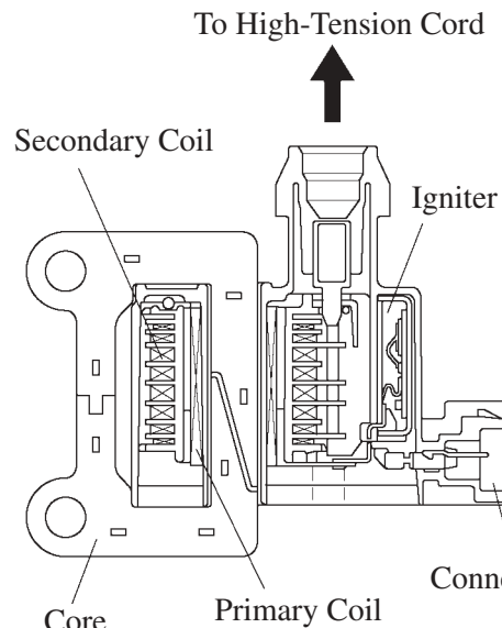
Ignition Coil Cross Section
