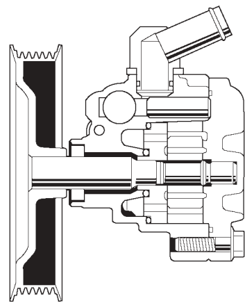
2UZ-FE Engine Model for Europe
