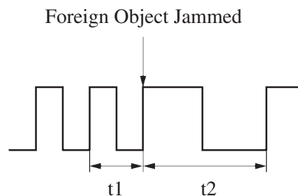
Output Pulse Signal
