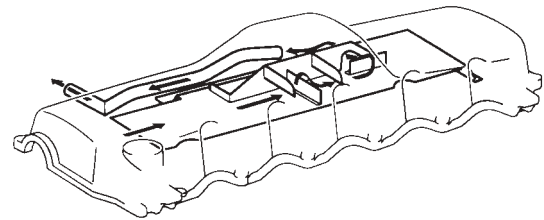
Blowby Gas Flow
