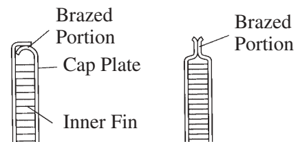
Ordinary Drawn Cup
