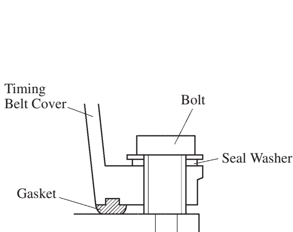
Timing Belt Cover Installation Portion
