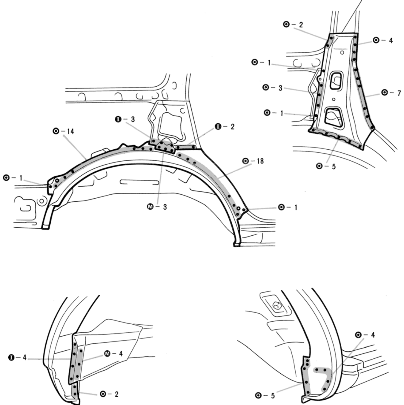
Roof Side Inner to Wheel Housing Brace
