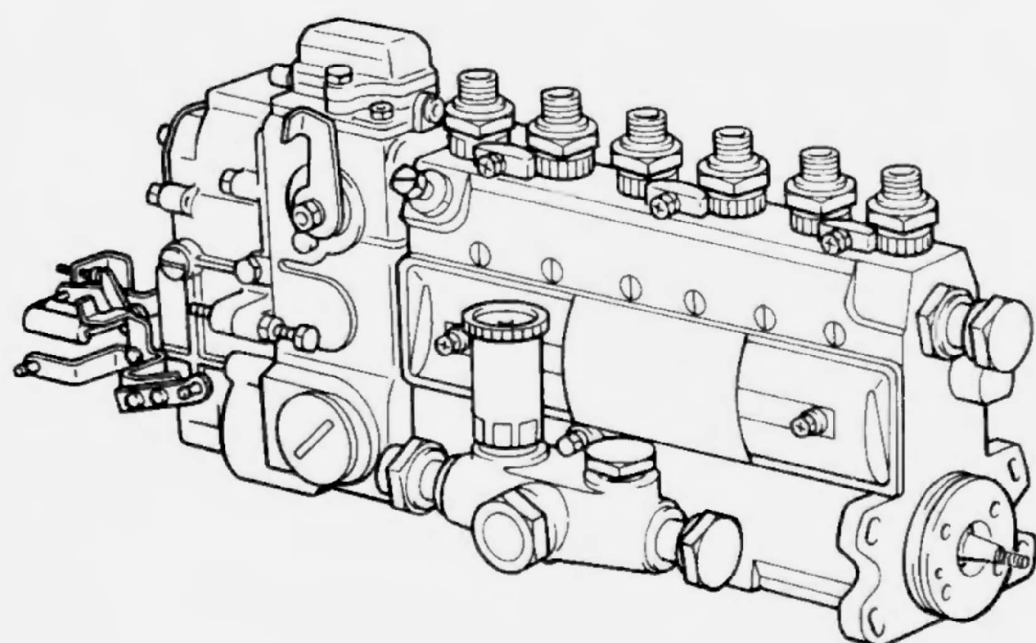
INJECTION PUMP WITH MECHANICAL GOVERNOR FOR 2H ENGINE
