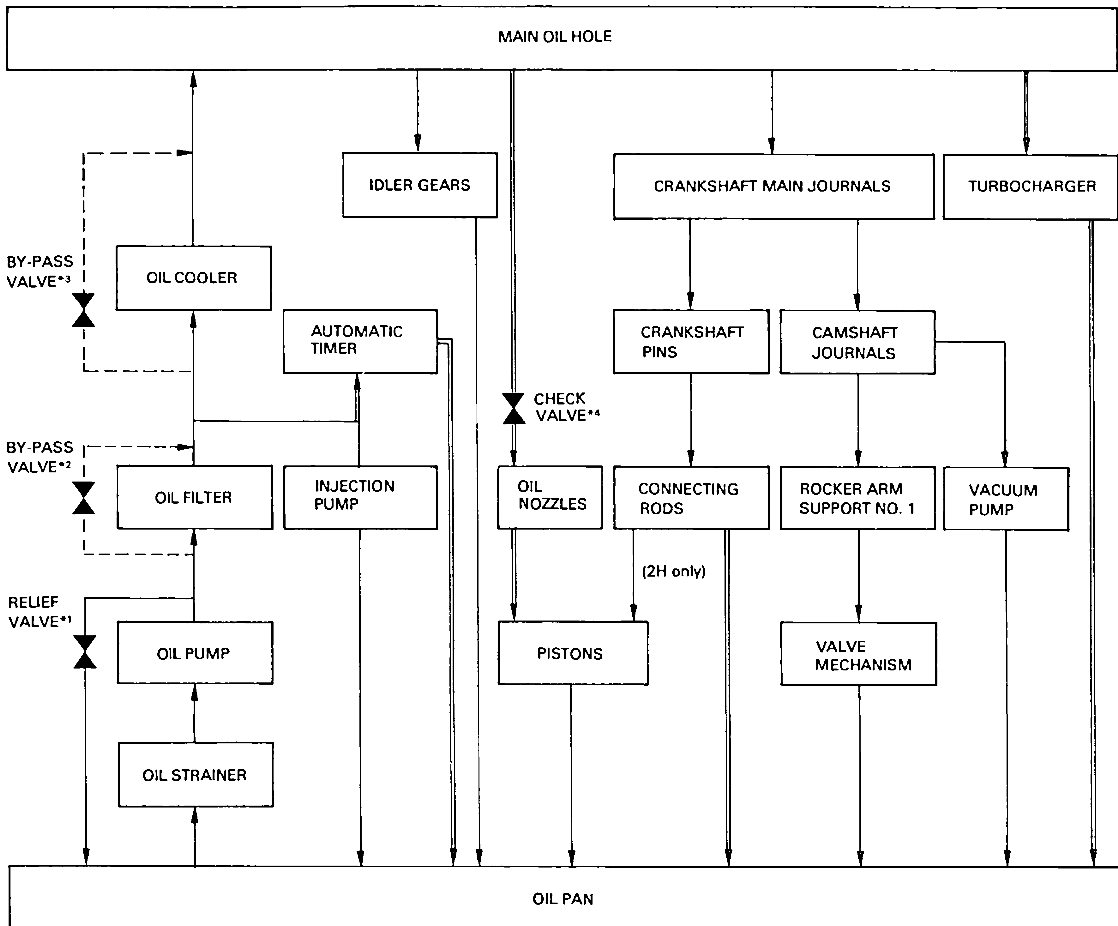
LUBRICATION CIRCUITRY
