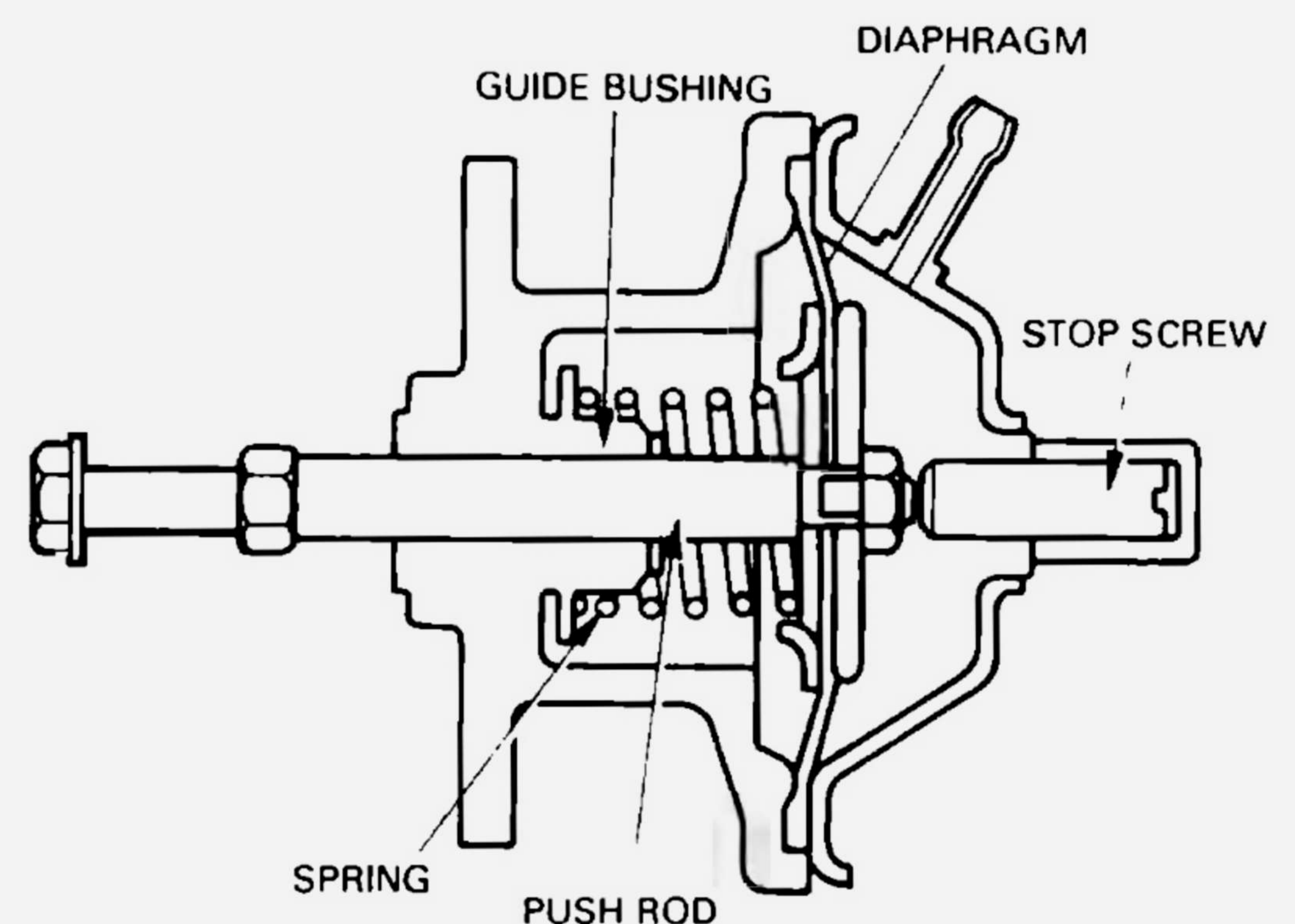
COMPONENTS OF MECHANICAL GOVERNOR FOR 12H-T
