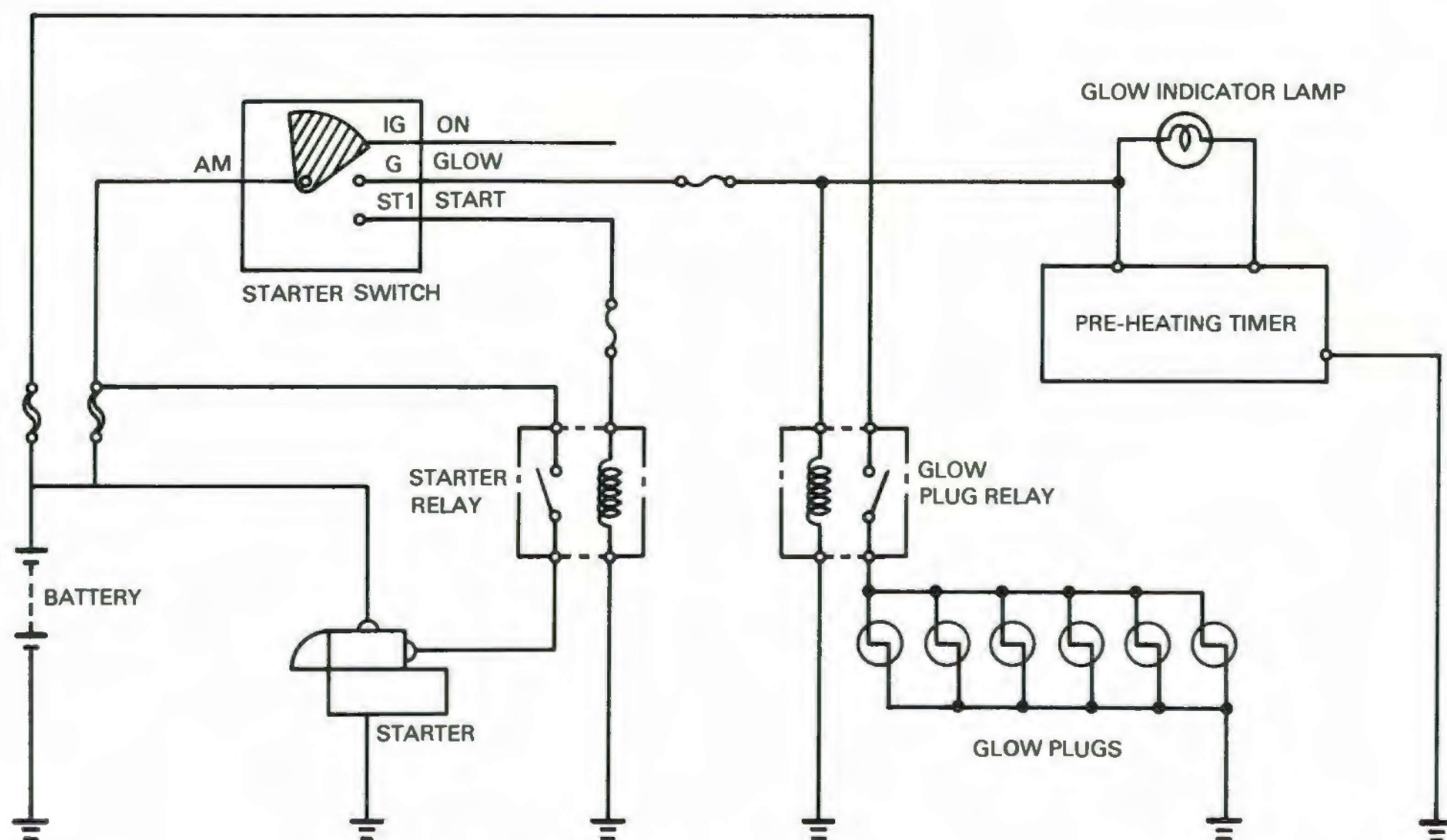
ELECTRICAL CIRCUITRY OF FIXED-DELAY TYPE
