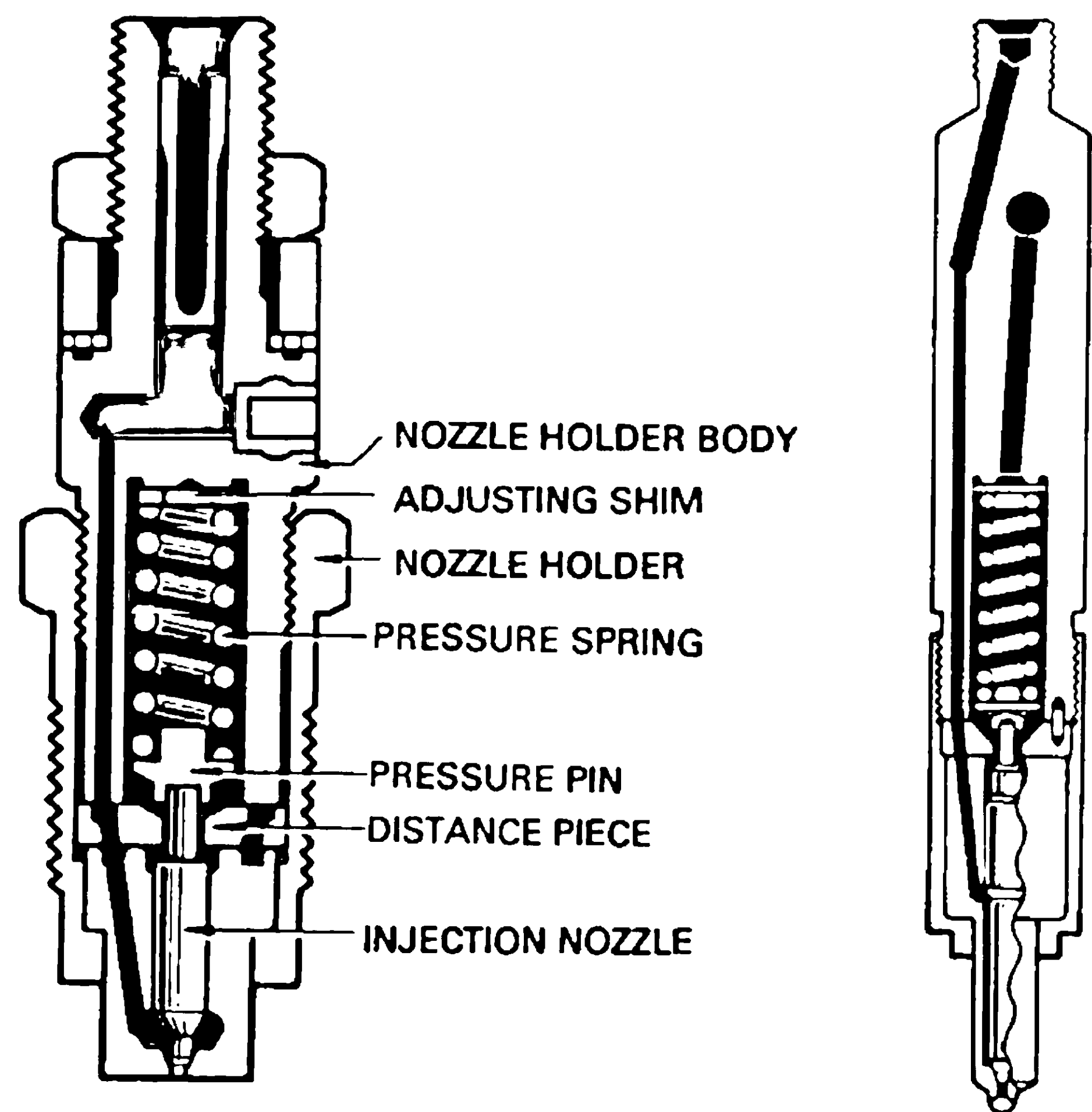
INJECTION NOZZLE FOR 2H
