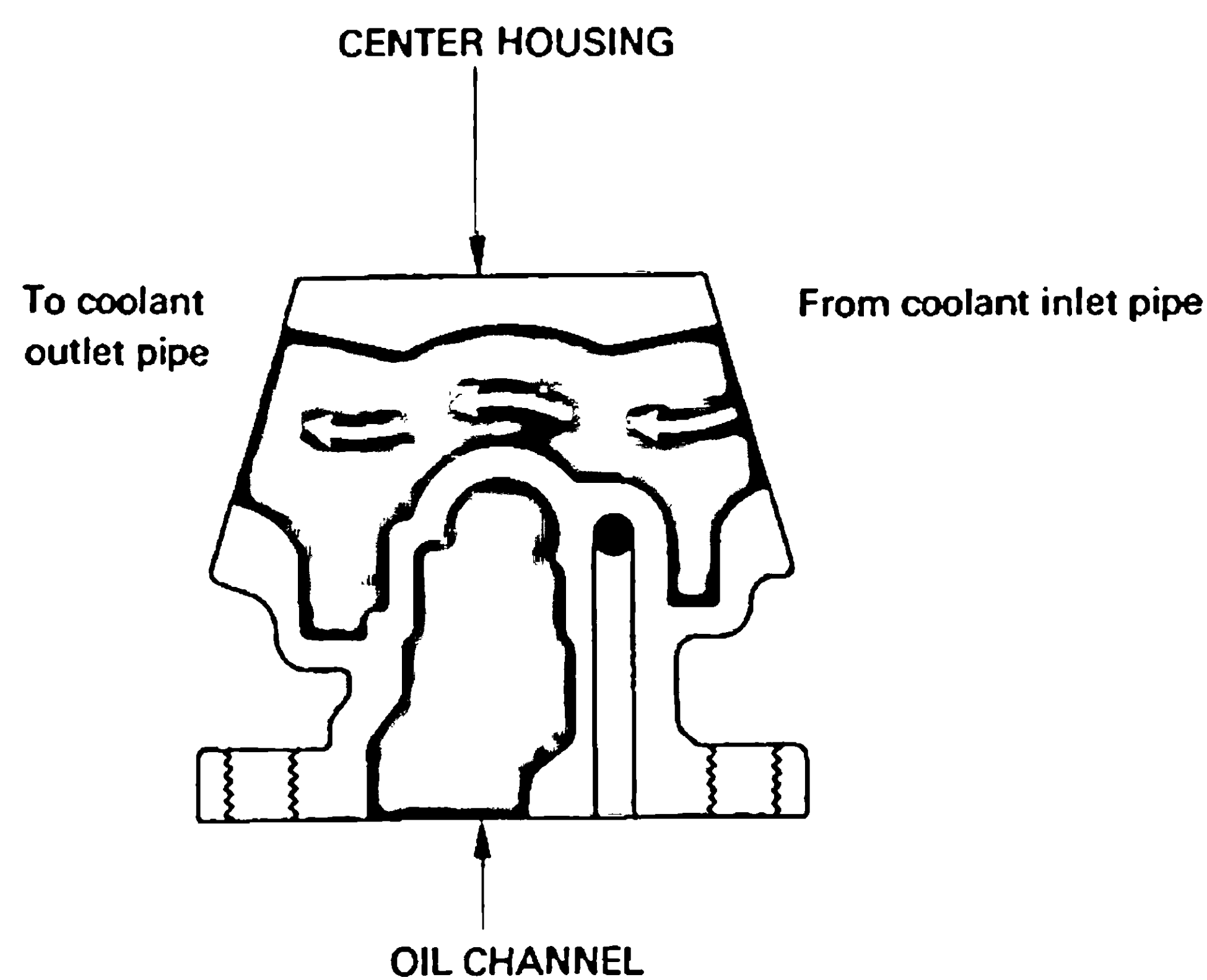
CUT-AWAY VIEW A-A (in illustration at left)
