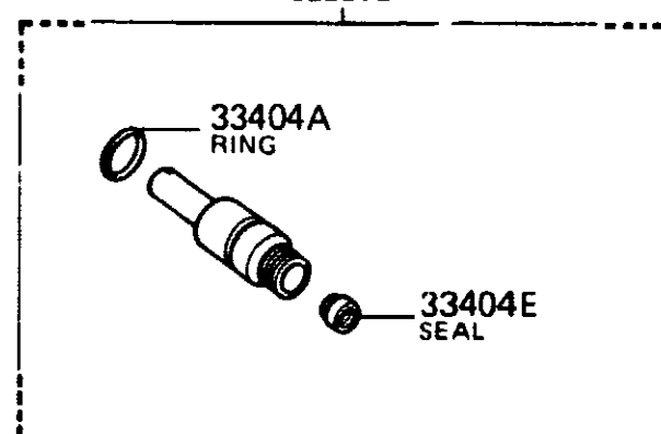
33404 SLEEVE
