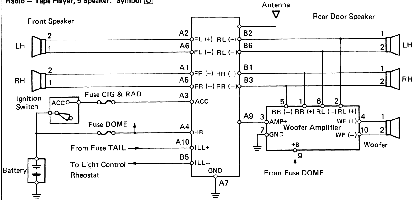
Woofer Amplifier
