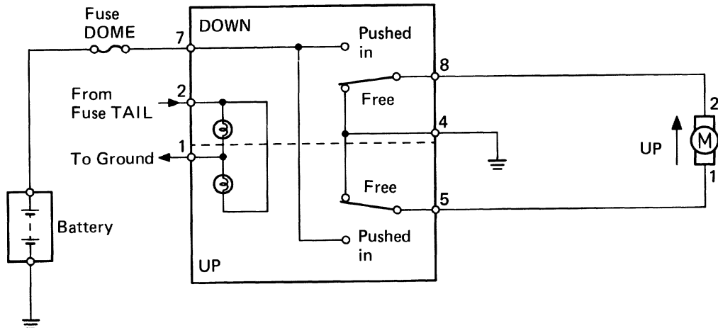
Antenna Motor
