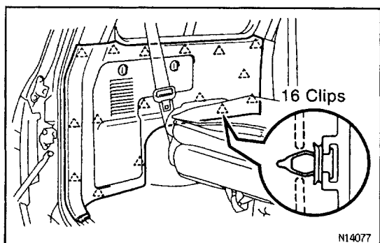
(e) Quarter trim (LH)
