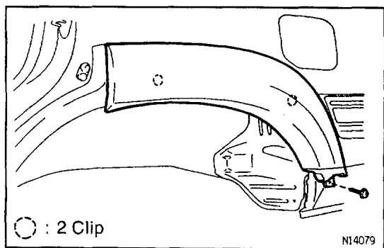
(b) Remove the screw.
