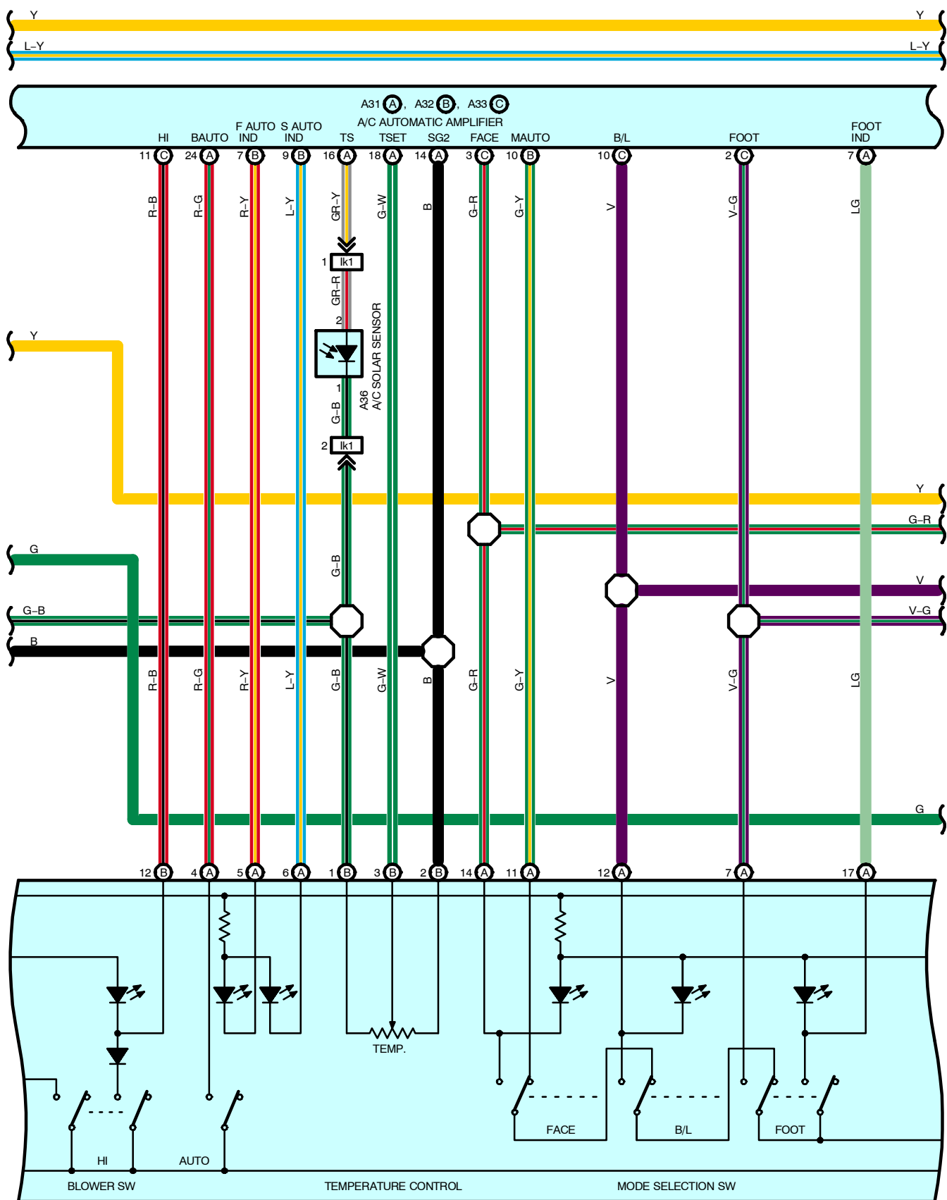
H10 (A), H11 (B) HEATER CONTROL SW AND A/C SW
