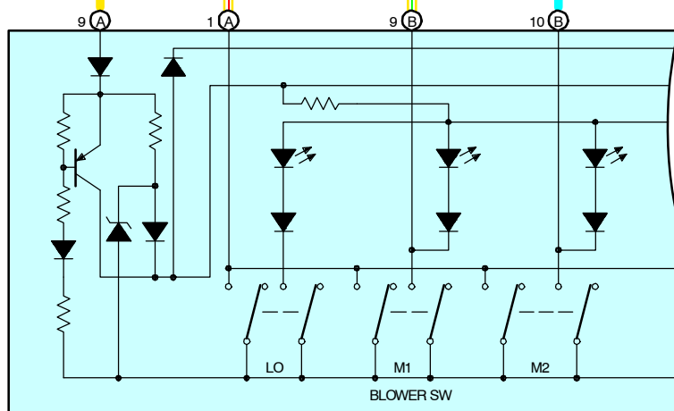
HEATER CONTROL SW AND A/C SW
