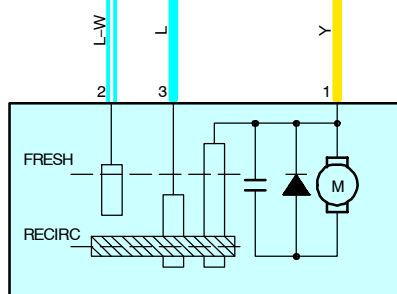
A14 AIRINLET CONTROL SERVO MOTOR
