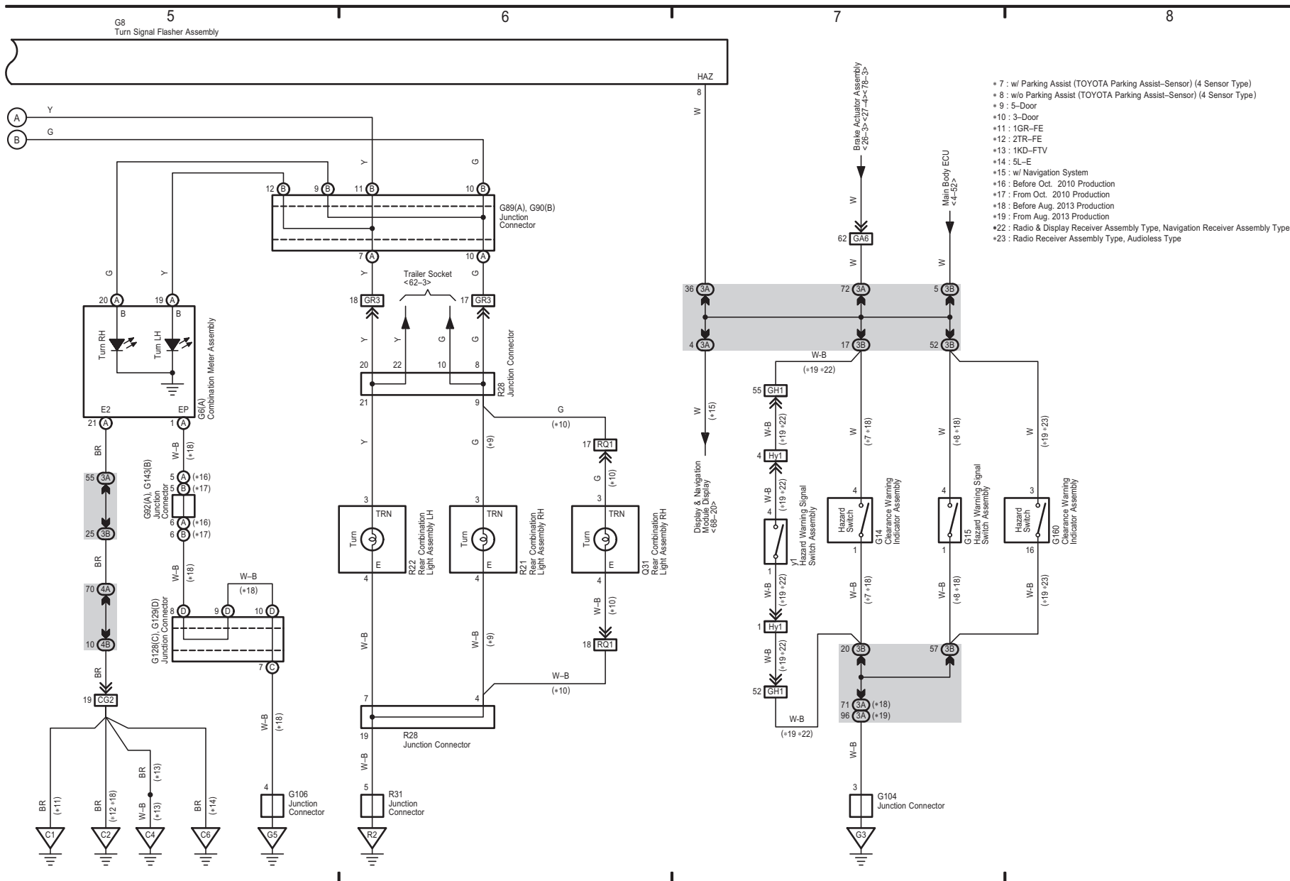
Turn Signal and Hazard Warning Light (RHD)
