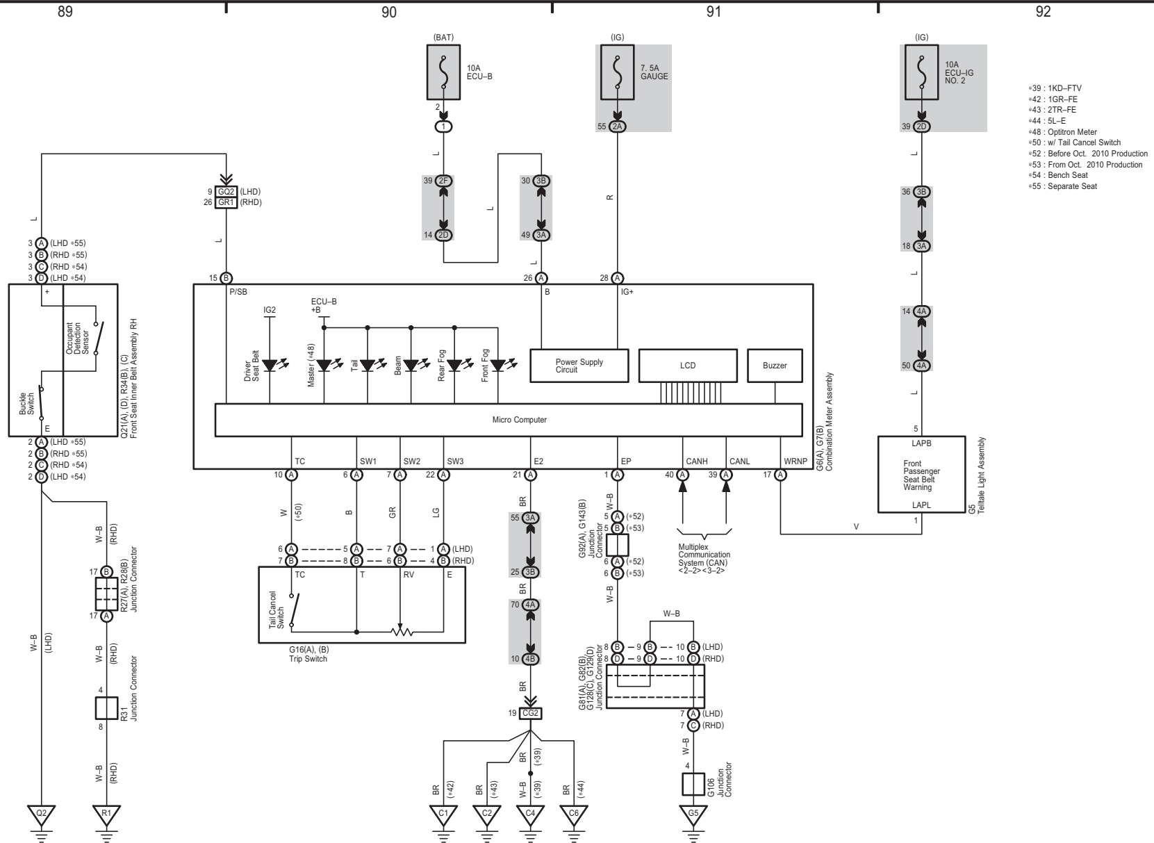
Multiplex Communication System (Body Control) (Before Aug. 2013 Production)
