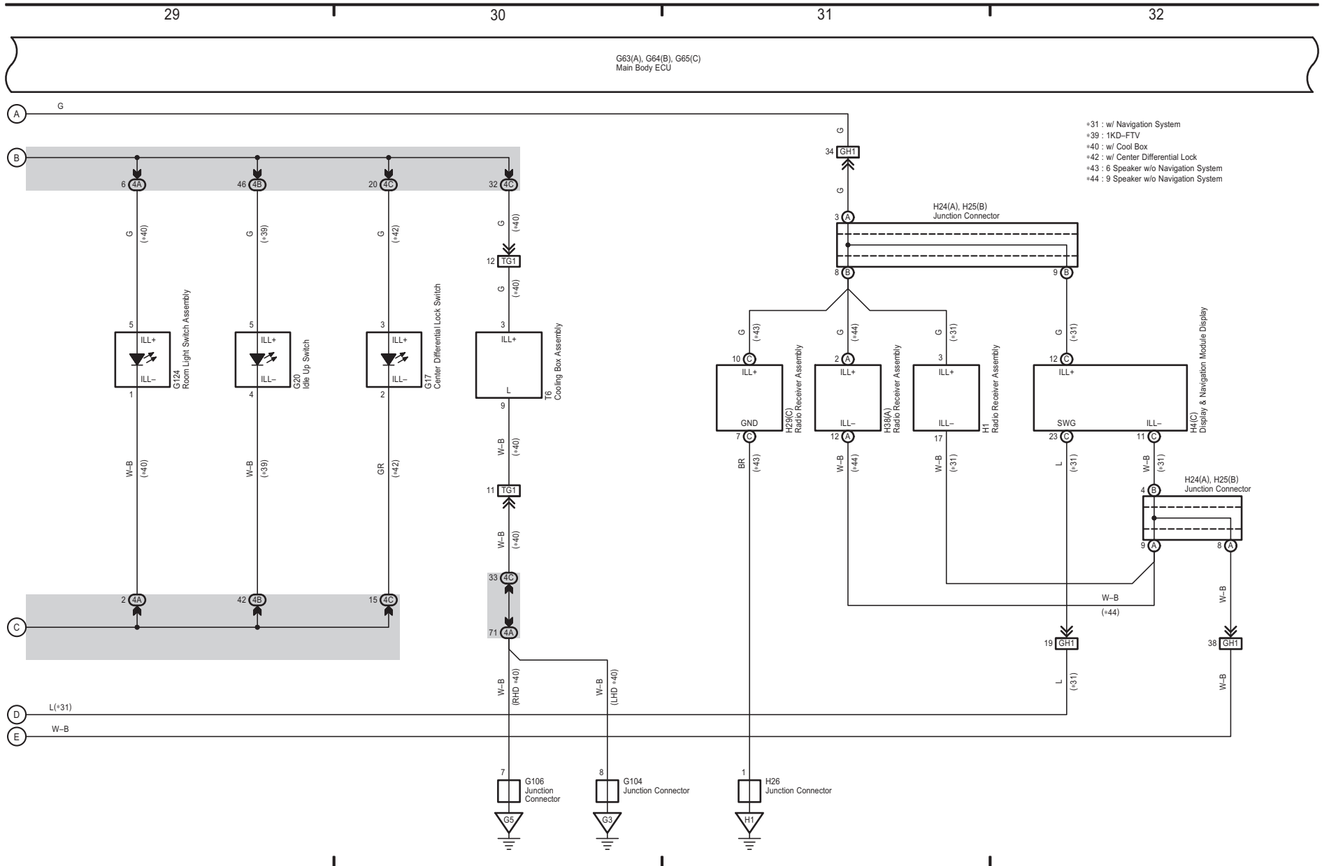
Multiplex Communication System (Body Control) (Before Aug. 2013 Production)
