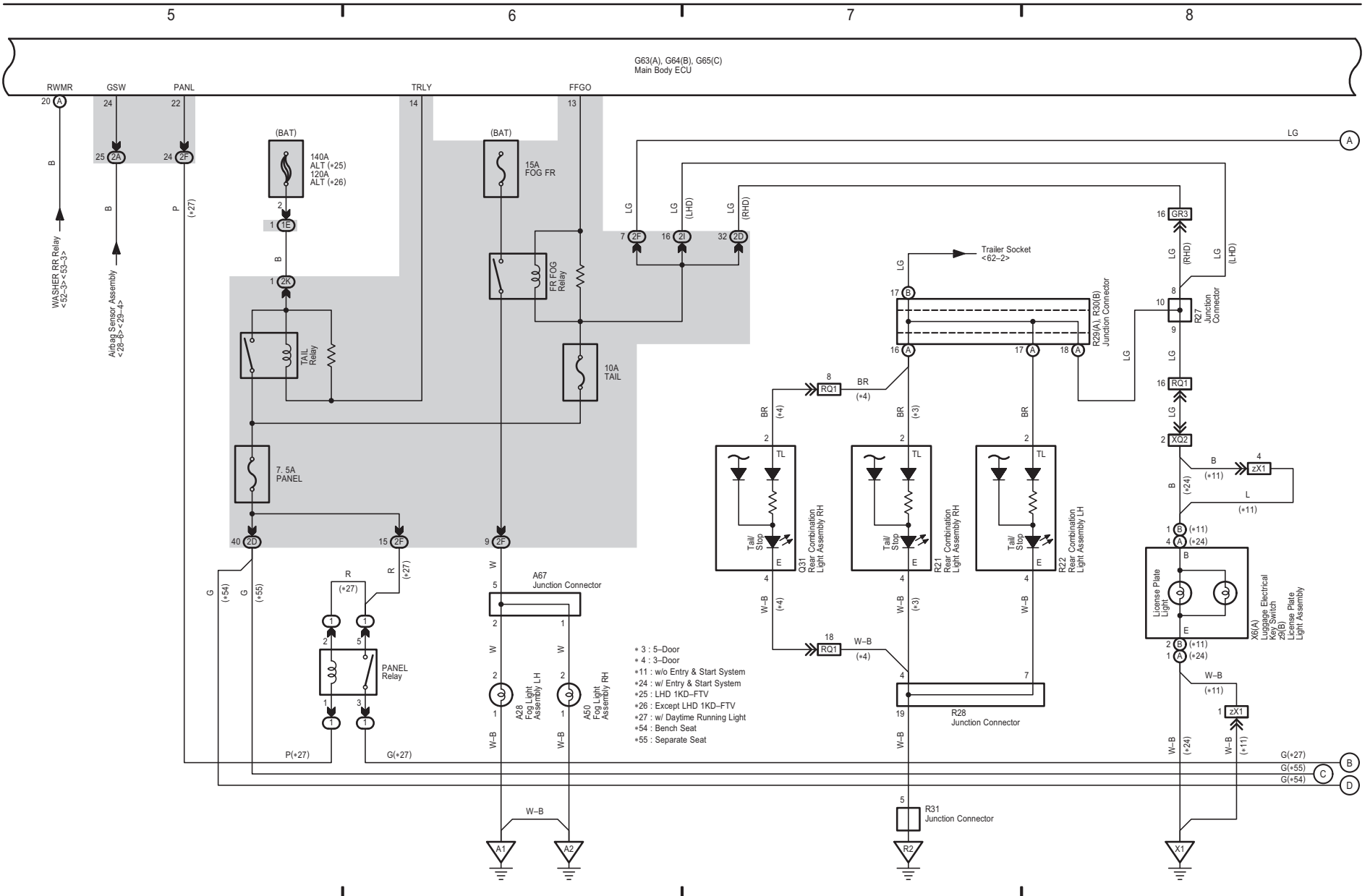
Multiplex Communication System (Body Control) (Before Aug. 2013 Production)
