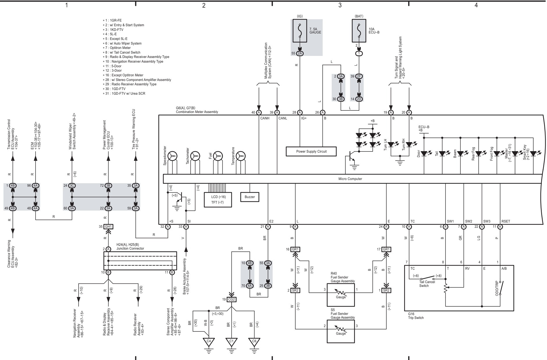
Combination Meter (RHD) (From Jun. 2015 until Aug. 2017 Production)
