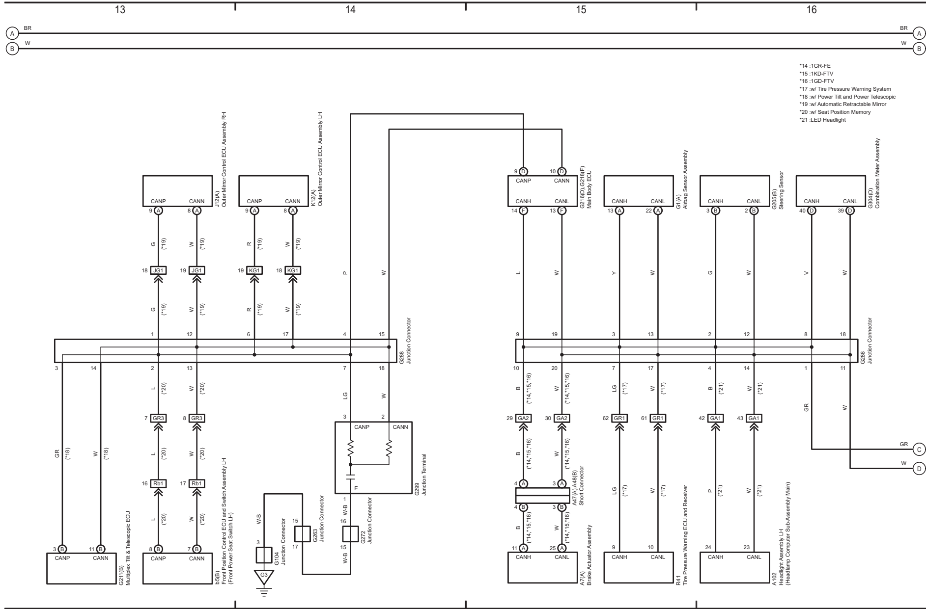
Multiplex Communication System (CAN LHD 1GR-FE, 2TR-FE, 1KD-FTV, 1GD-FTV) (From Aug. 2017 Production)
