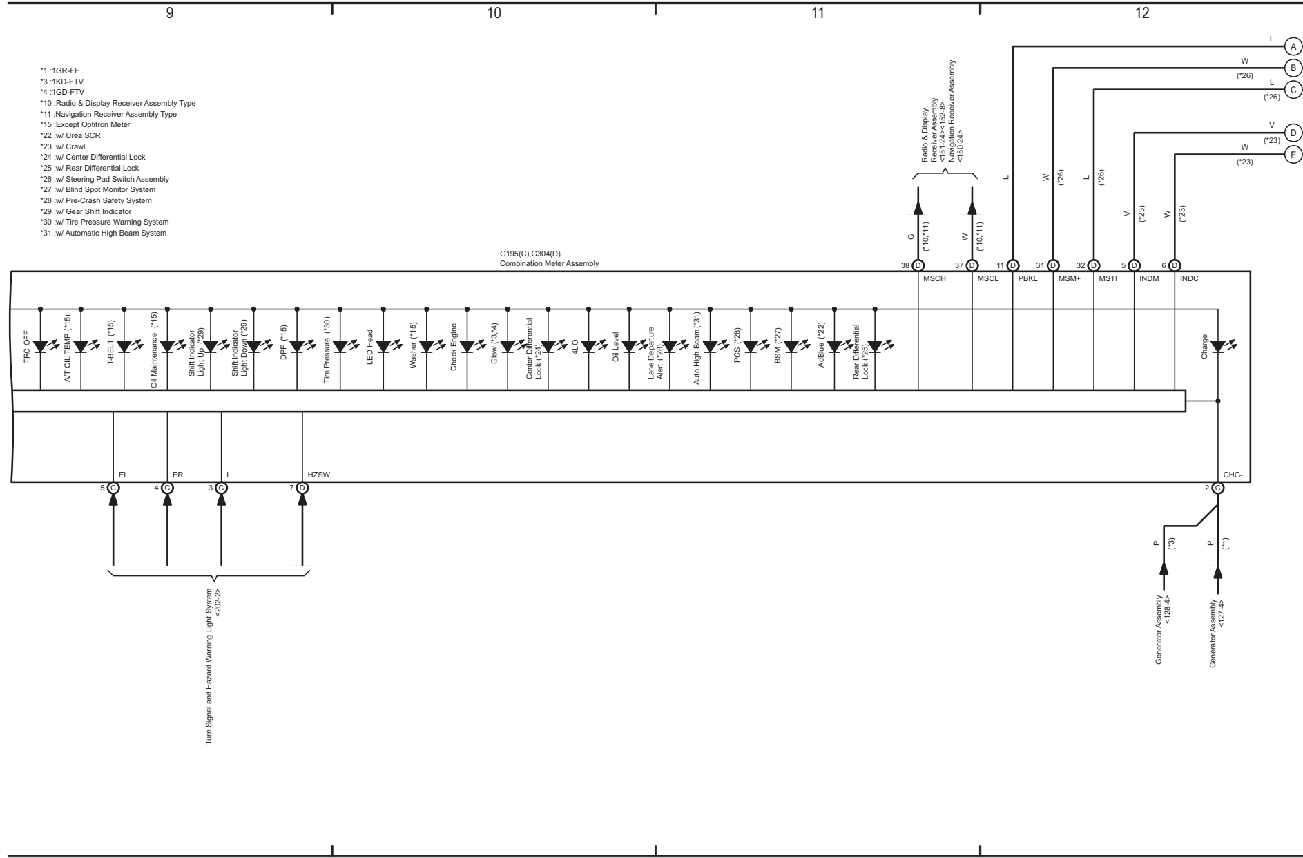
Combination Meter (LHD 1GR-FE, 2TR-FE, 1KD-FTV, 1GD-FTV) (From Aug. 2017 Production)
