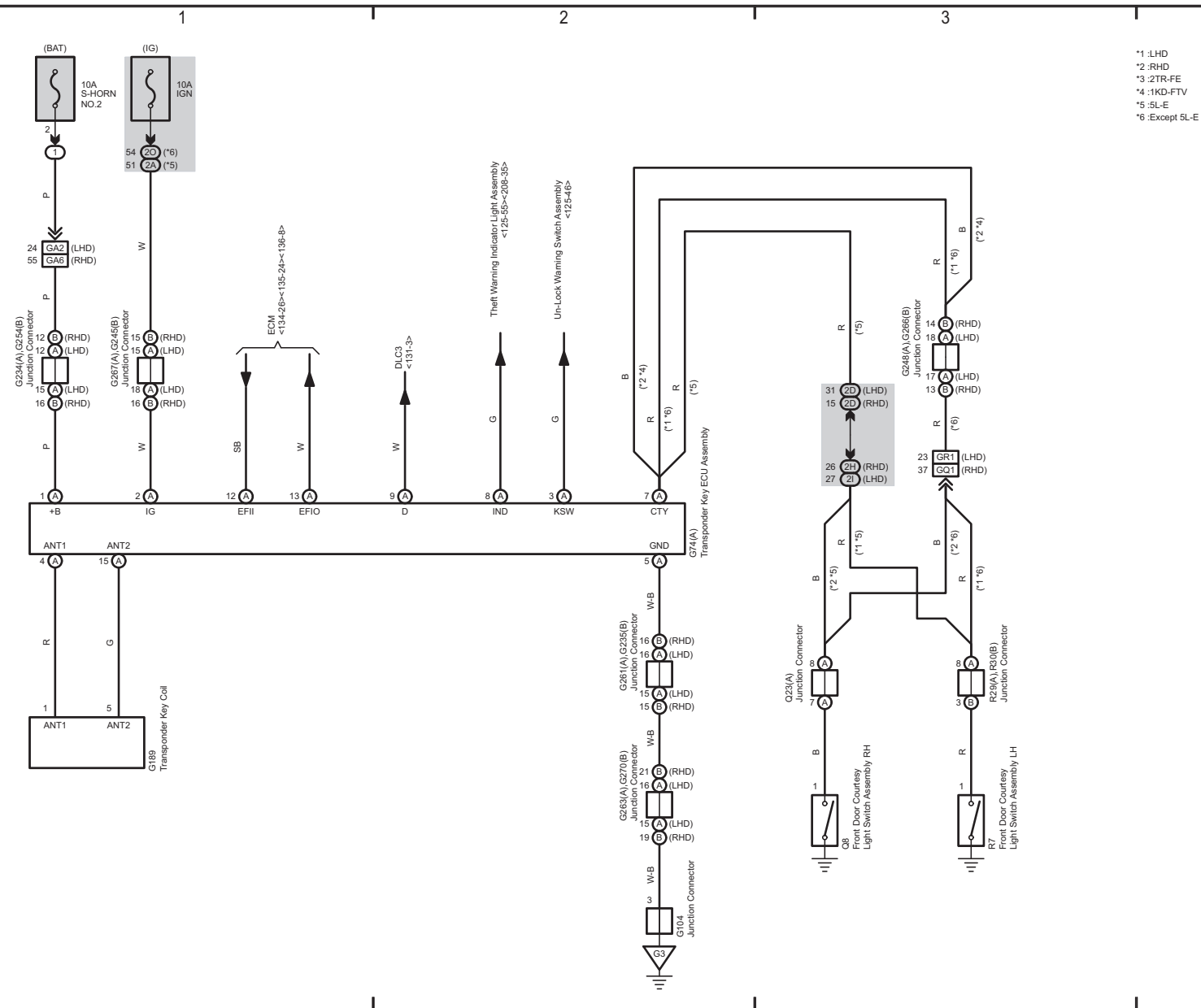
Engine Immobiliser System (w/o Entry &amp; Start System) (From Aug. 2017 Production)
