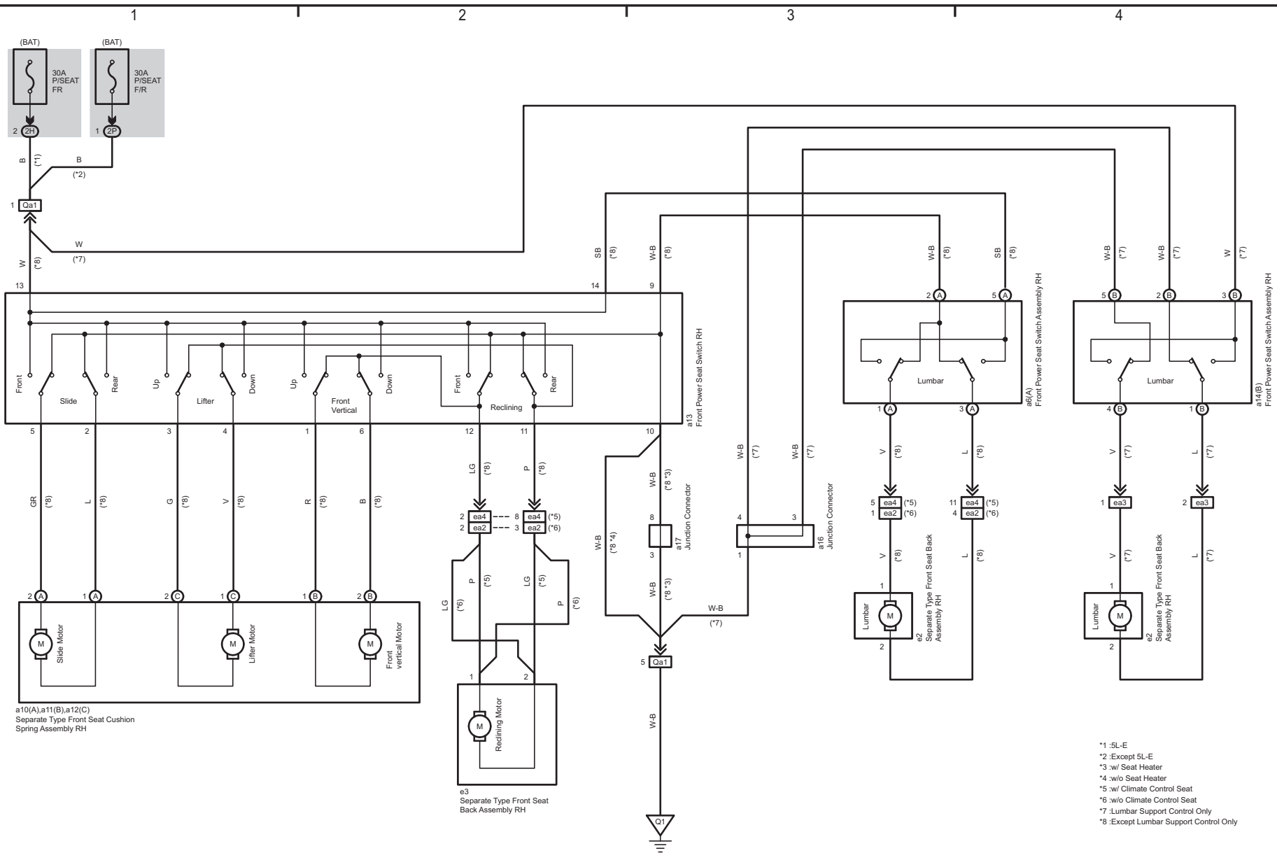
Power Seat (RHD Driver's Seat w/o Seat Position Memory) (From Aug. 2017 Production)
