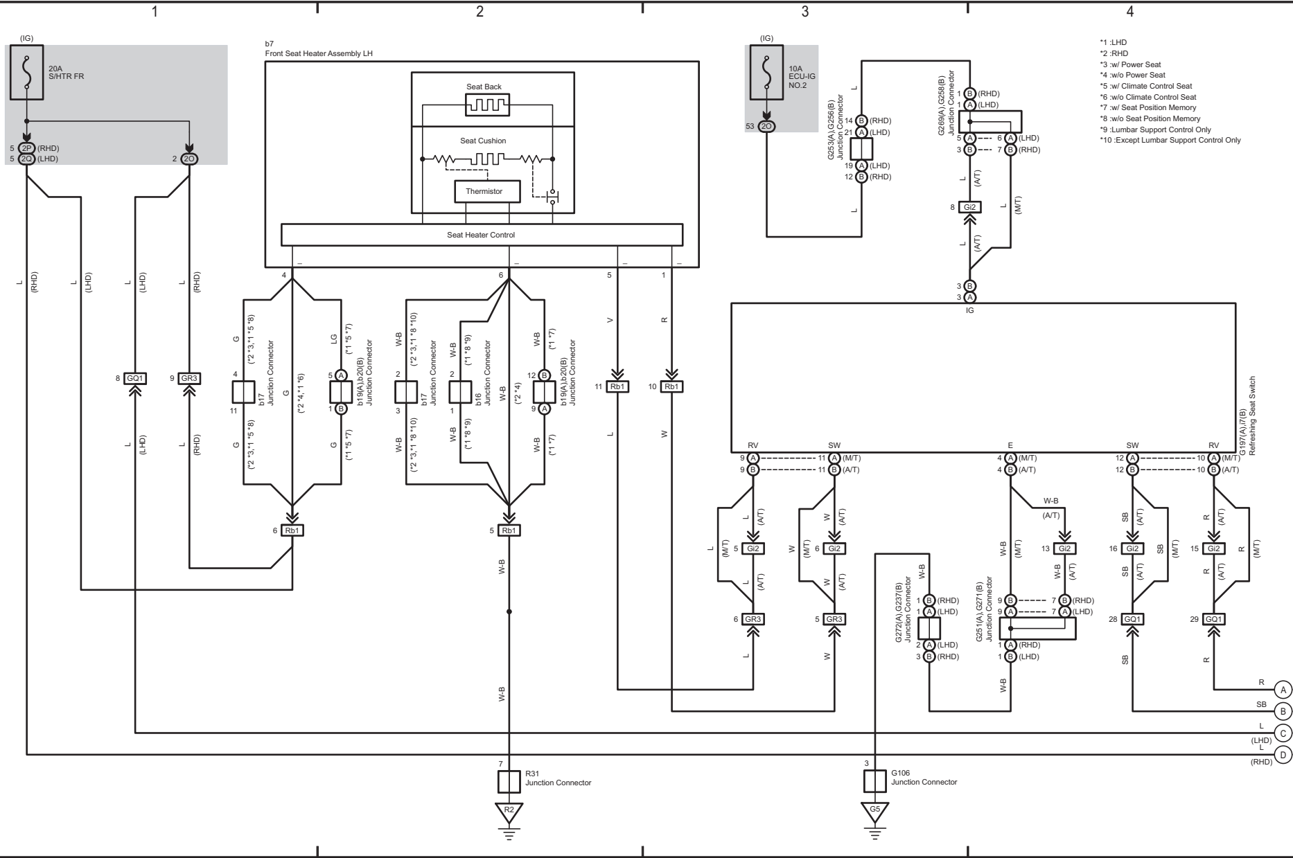
Seat Heater (Front) (From Aug. 2017 Production)
