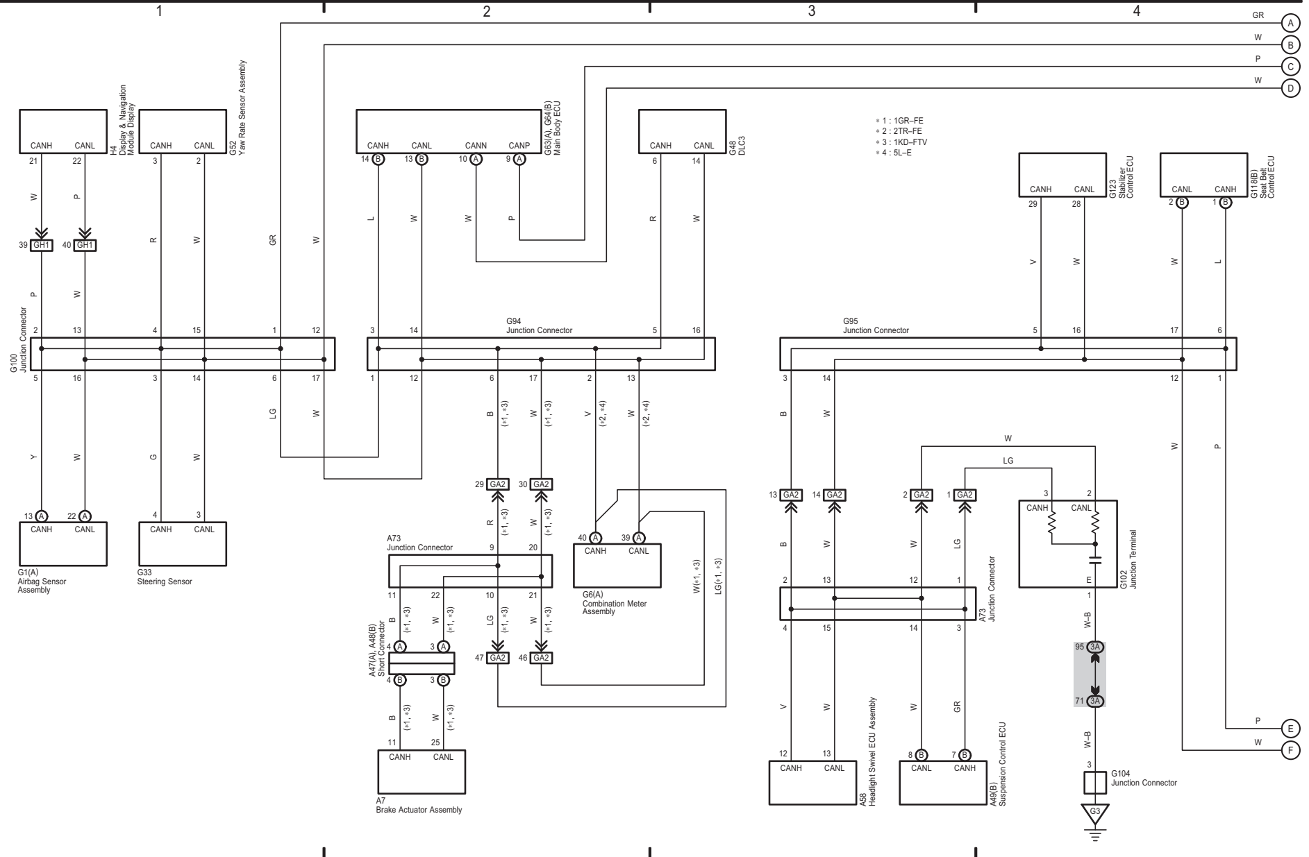
Multiplex Communication System (CAN LHD) (Before Aug. 2013 Production)
