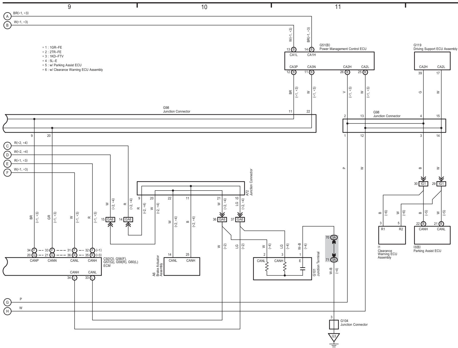
Multiplex Communication System (CAN LHD) (Before Aug. 2013 Production)
