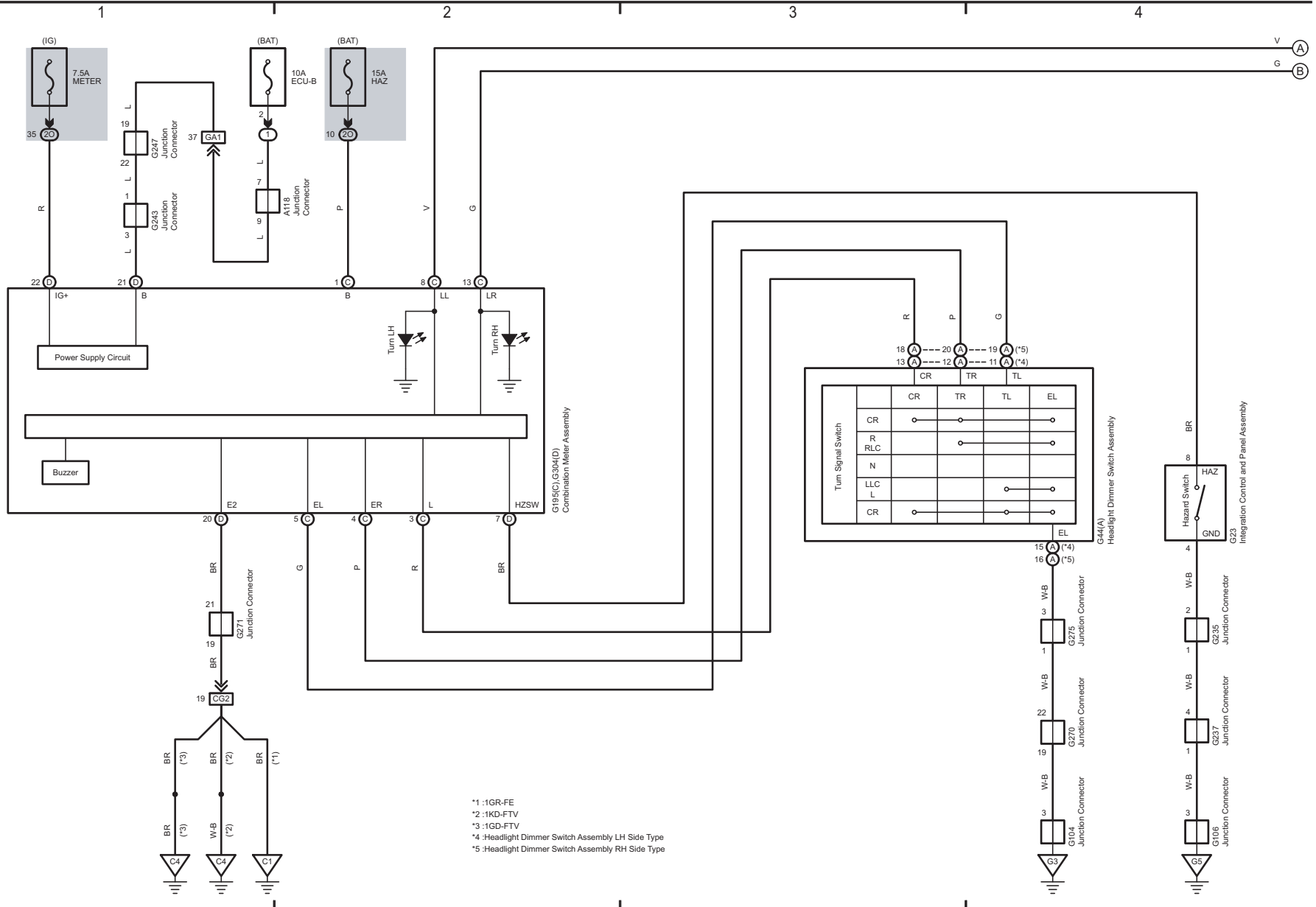
Turn Signal and Hazard Warning Light (RHD 1GR-FE, 1KD-FTV, 1GD-FTV) (From Aug. 2017 Production)
