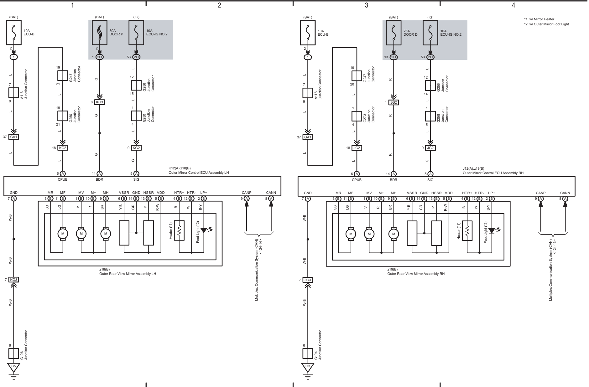
Mirror Heater (RHD w/ Automatic Retractable Mirror) (From Aug. 2017 Production), Remote Control Mirror (RHD w/ Automatic Retractable Mirror) (From Aug. 2017 Production)
