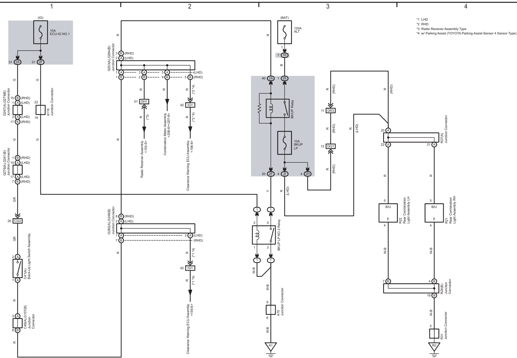
Back-Up Light (5L-E) (From Aug. 2017 Production)
