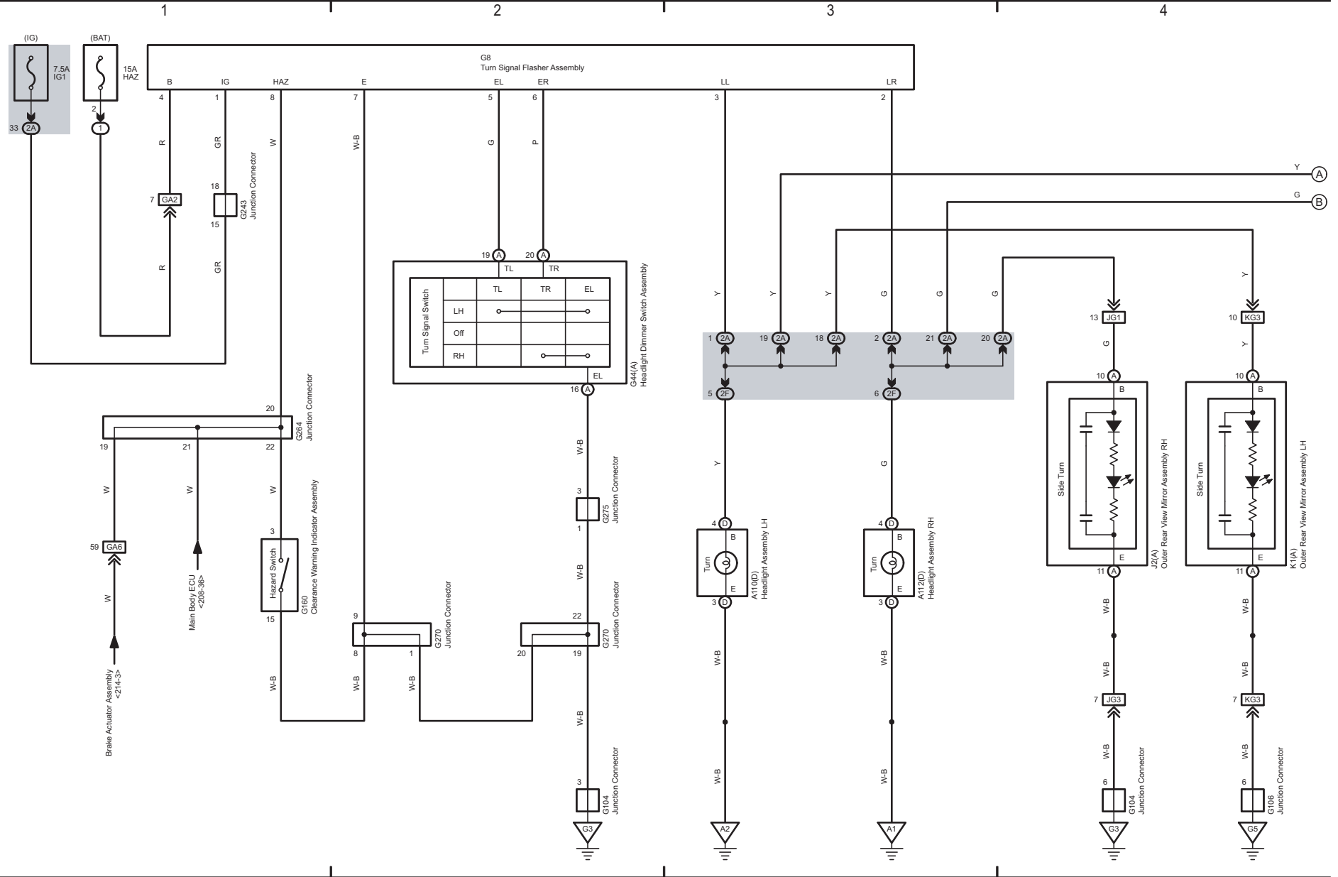
Turn Signal and Hazard Warning Light (RHD 5L-E) (From Aug. 2017 Production)
